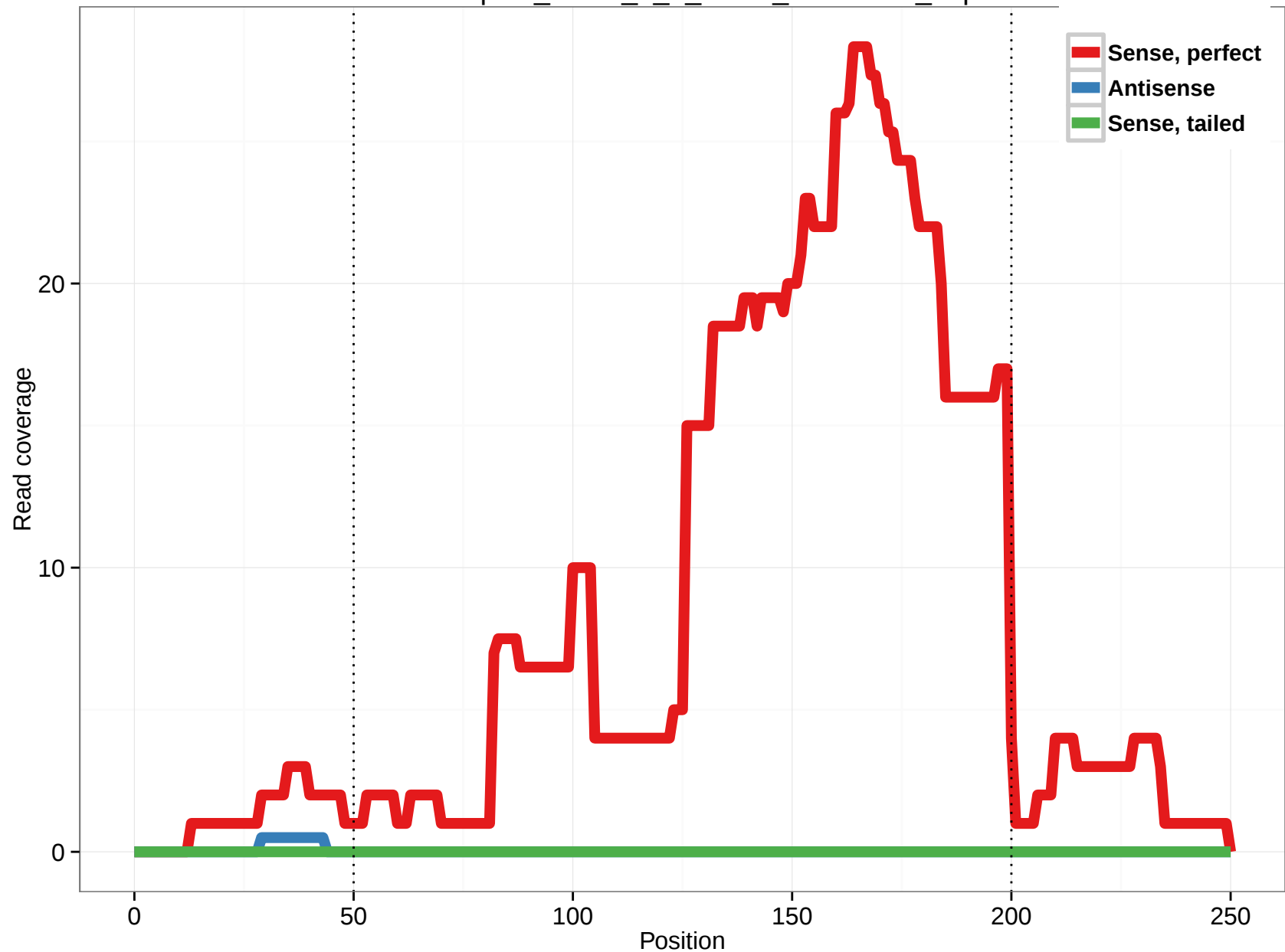
uc010apx.1_intron_9_0_chr14_64564865_f.3p
