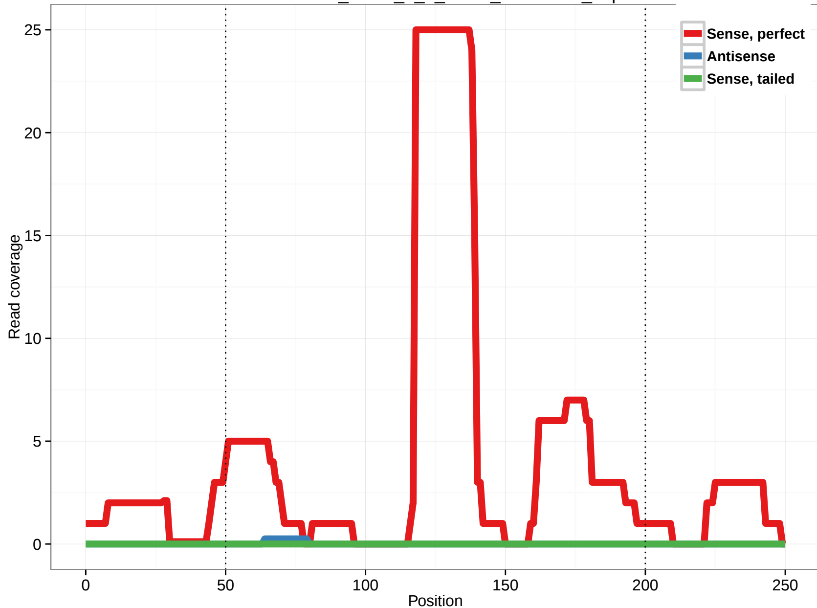
uc010alu.2_intron_1_0_chr14_24838877_f.5p
