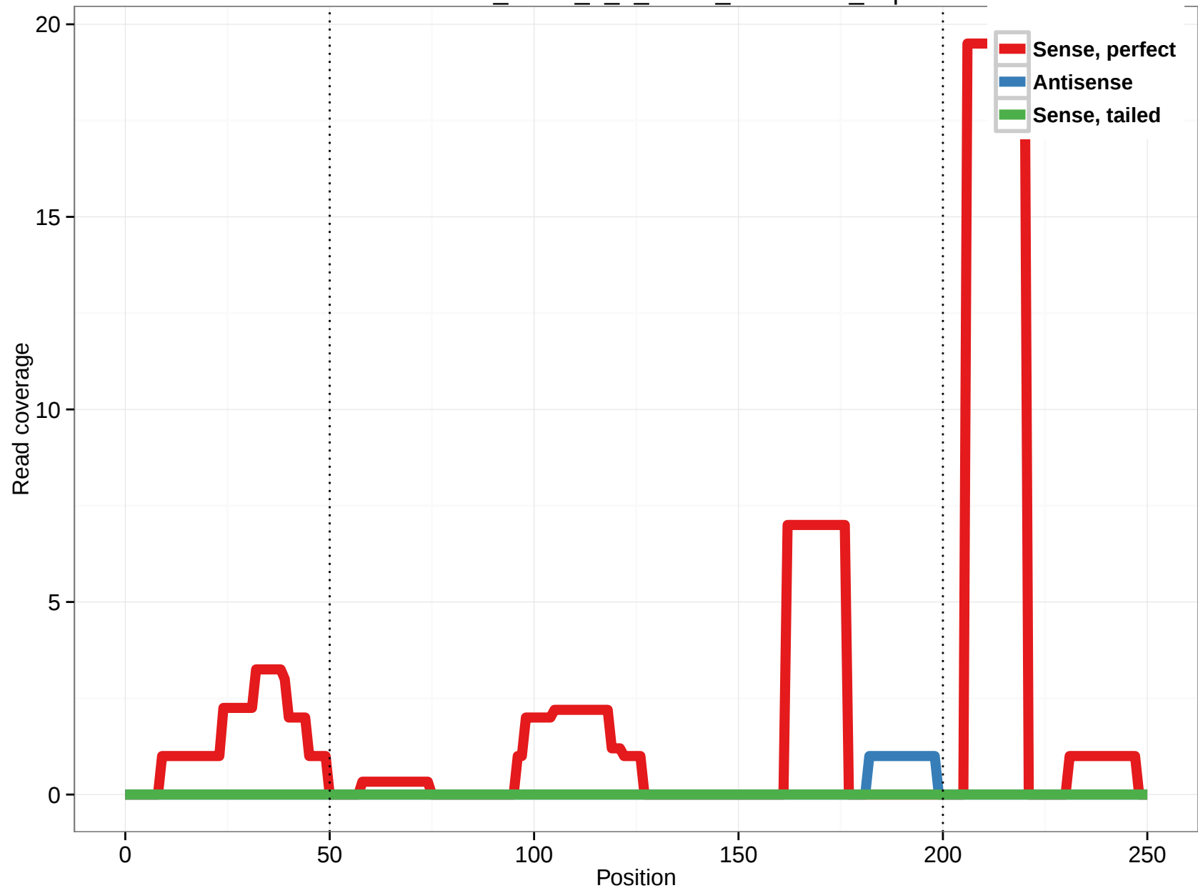
uc010als.2_intron_1_0_chr14_24837647_f.5p
