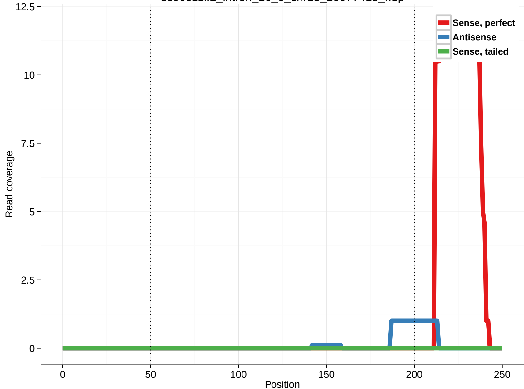
uc009zzl.2_intron_16_0_chr13_20077418_r.3p
