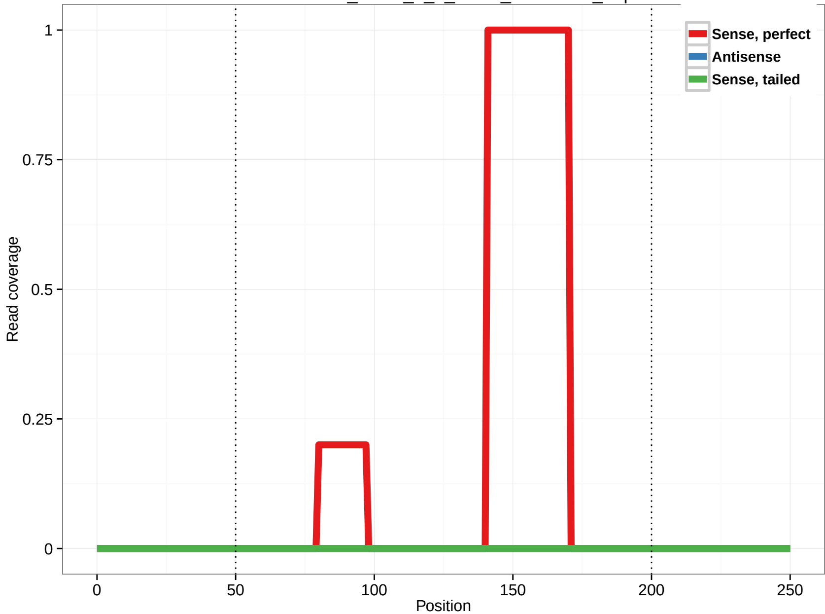
uc009zsh.2_intron_0_0_chr12_81653440_r.5p
