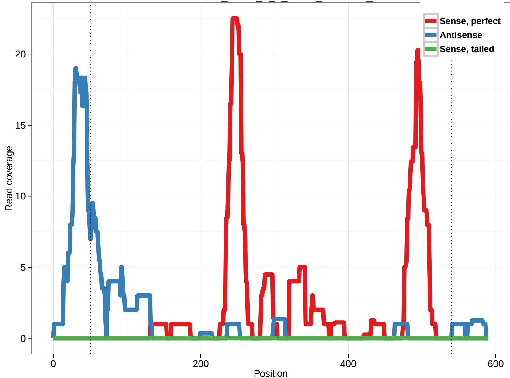
uc009zfu.1_intron_0_0_chr12_7342128_f
