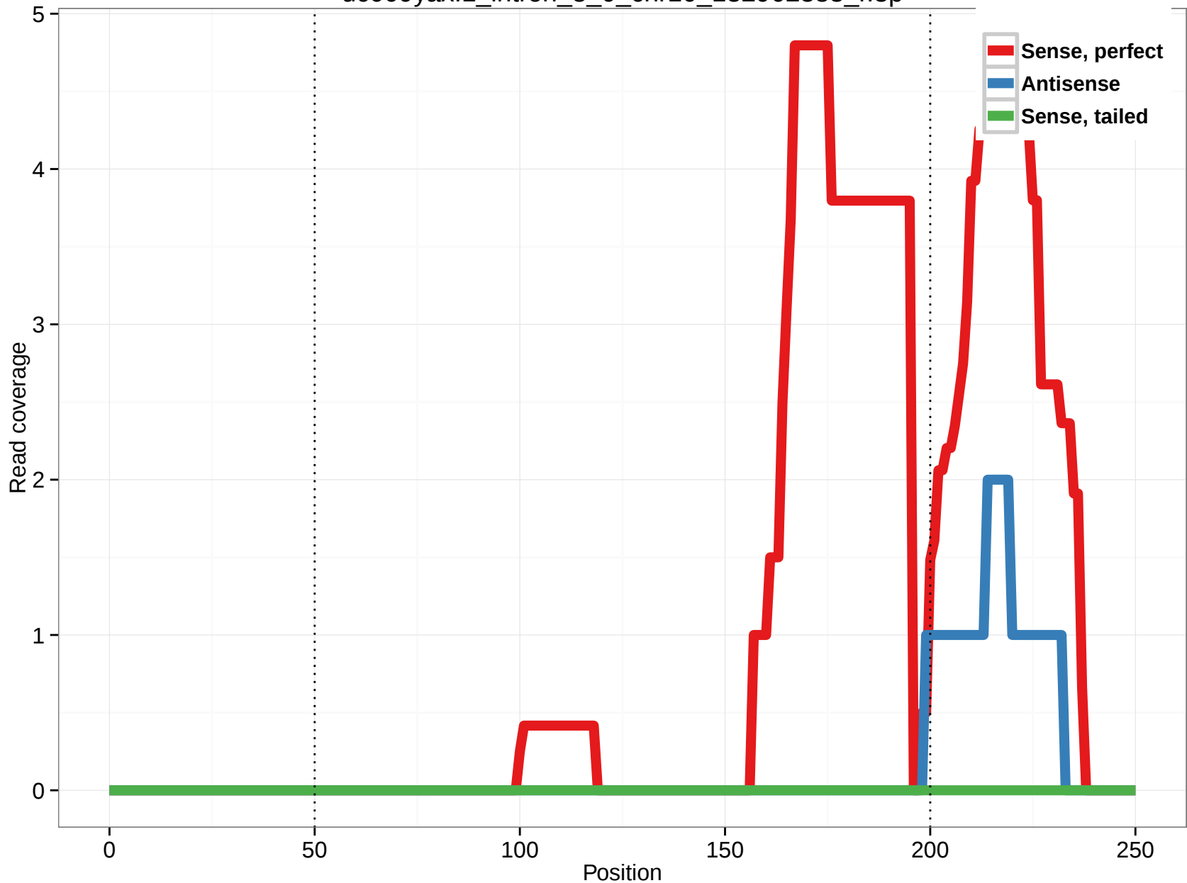
uc009yax.1_intron_8_0_chr10_132962383_r.3p
