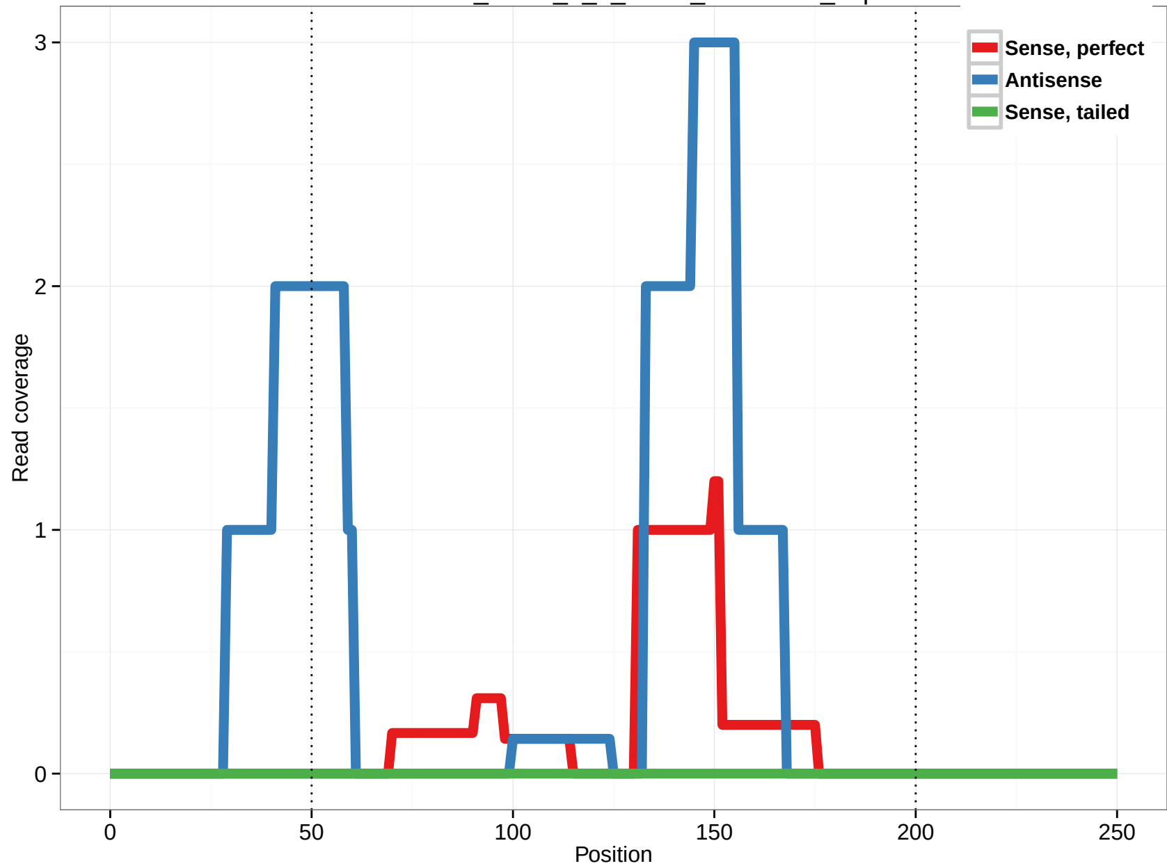
uc009xix.2_intron_3_0_chr10_11794254_f.5p
