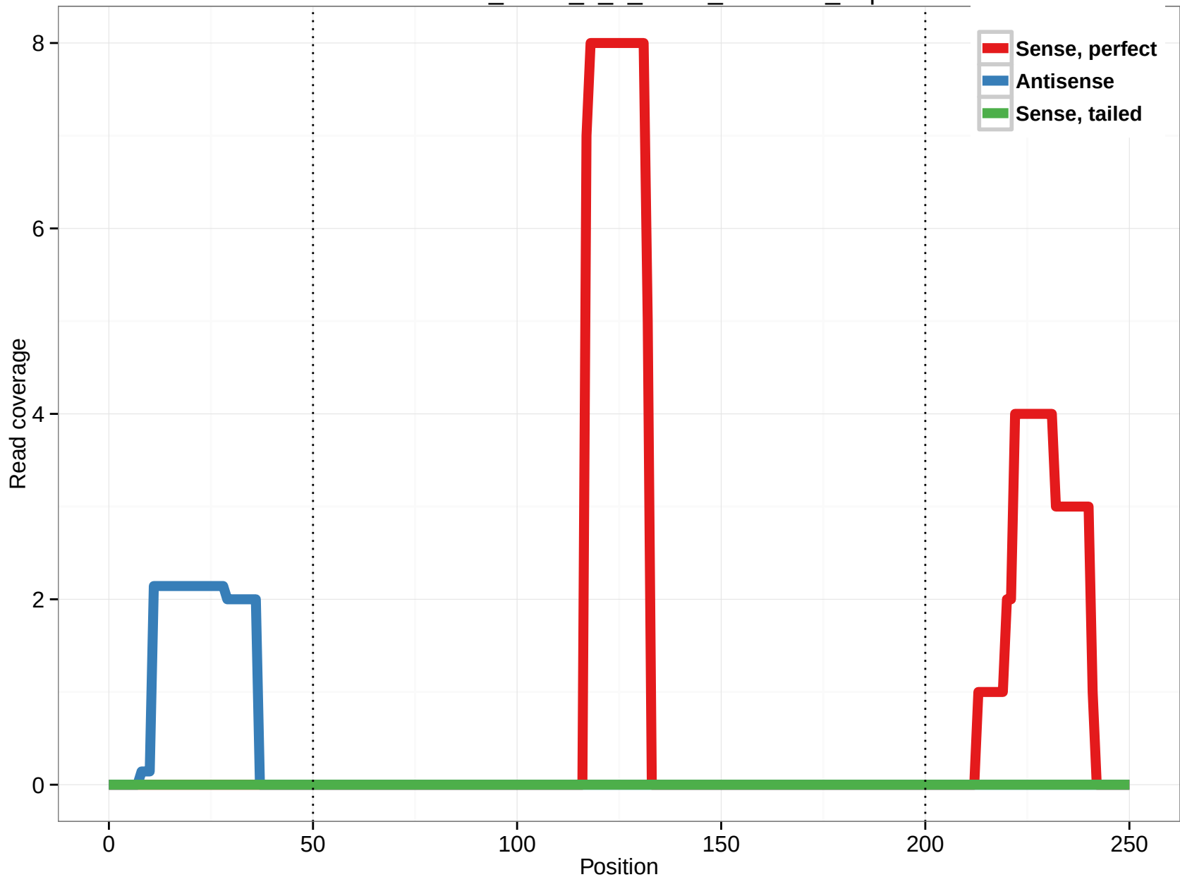
uc009xhz.2_intron_3_0_chr10_5202853_r.3p
