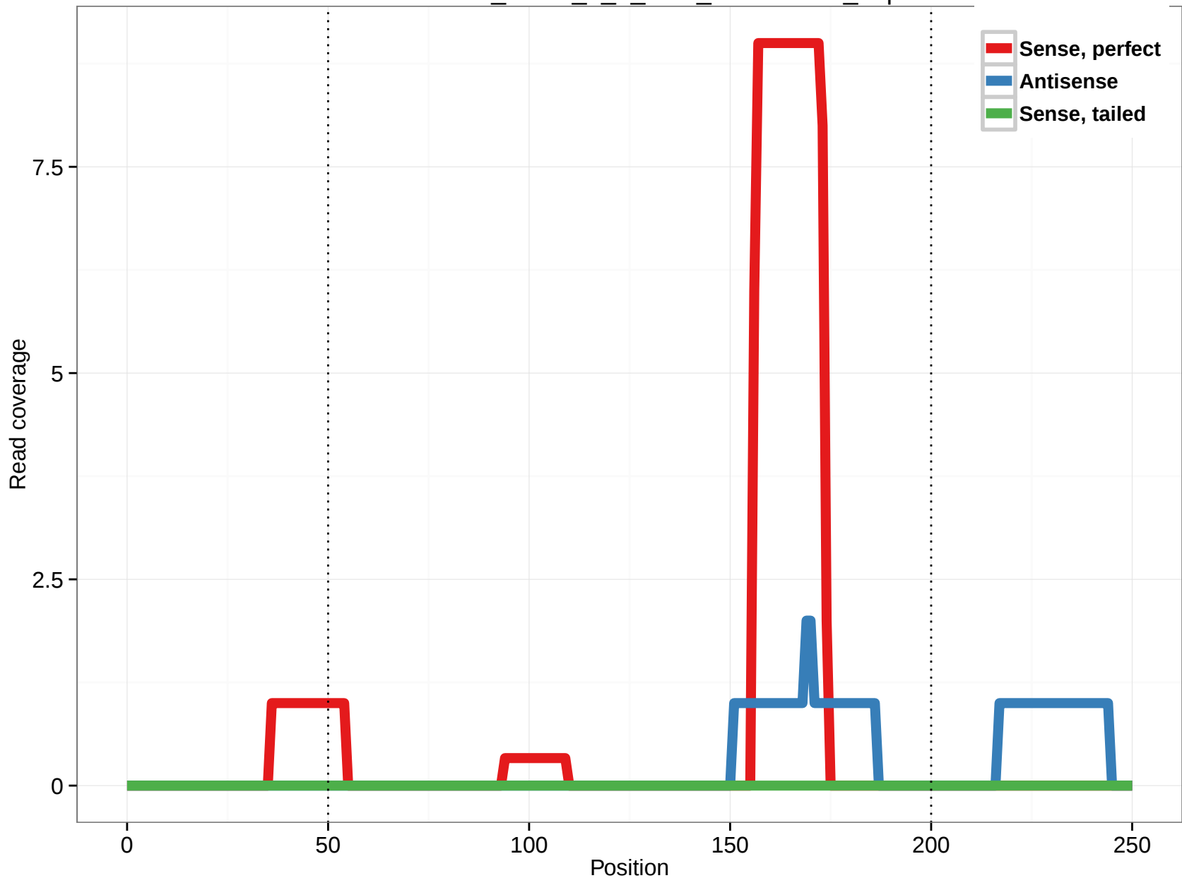
uc009xcx.2_intron_0_0_chr1_210501729_f.5p
