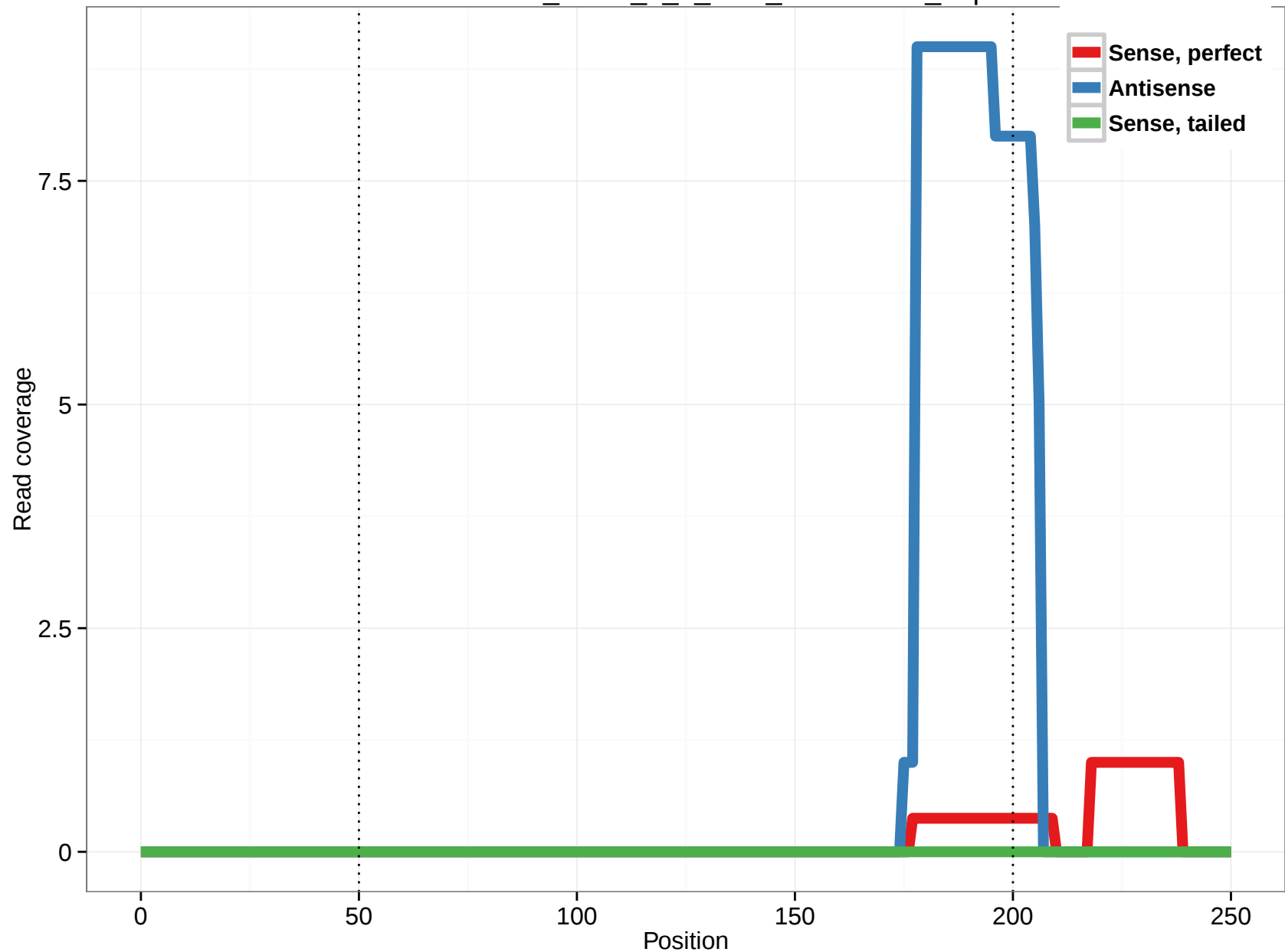
uc009wvm.2_intron_3_0_chr1_167853587_r.5p
