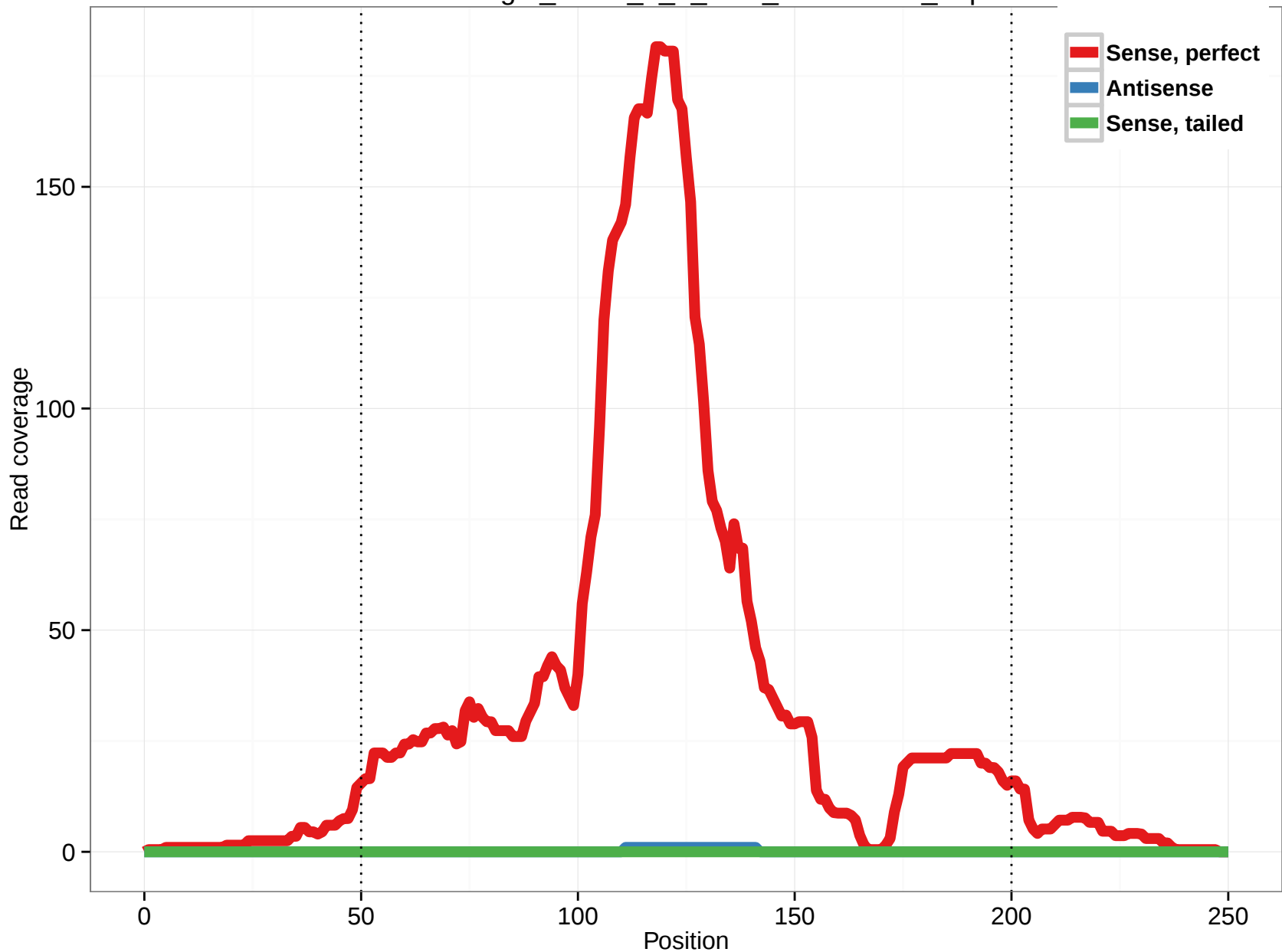
uc009wsg.2_intron_0_0_chr1_156712763_r.3p
