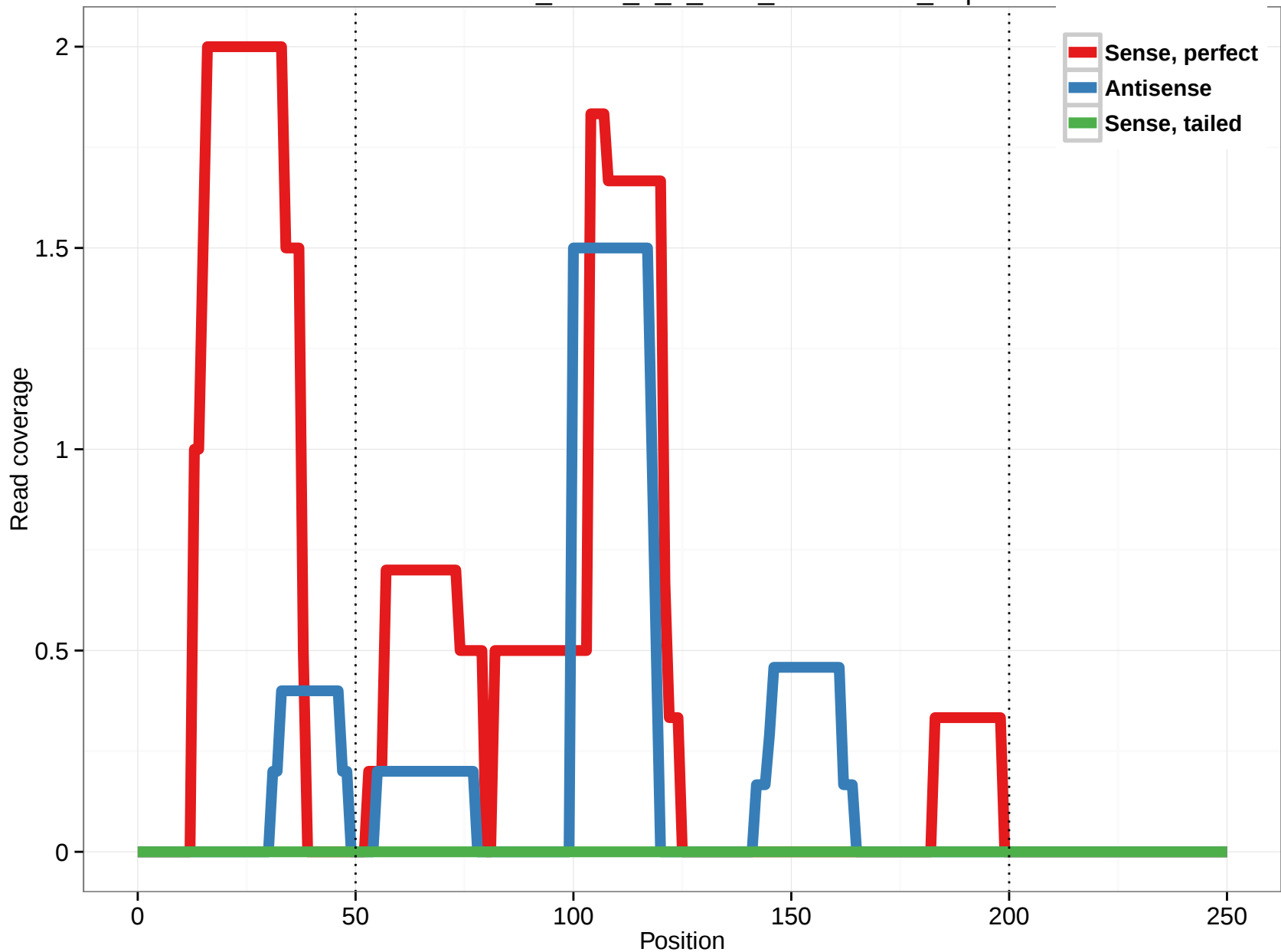
uc009whx.2_intron_1_0_chr1_143719187_r.5p
