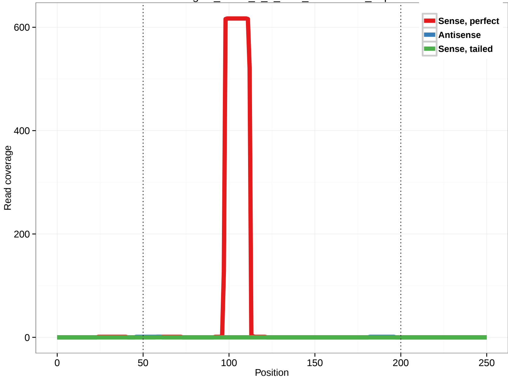
uc009wgz.2_intron_0_0_chr1_116381002_r.3p
