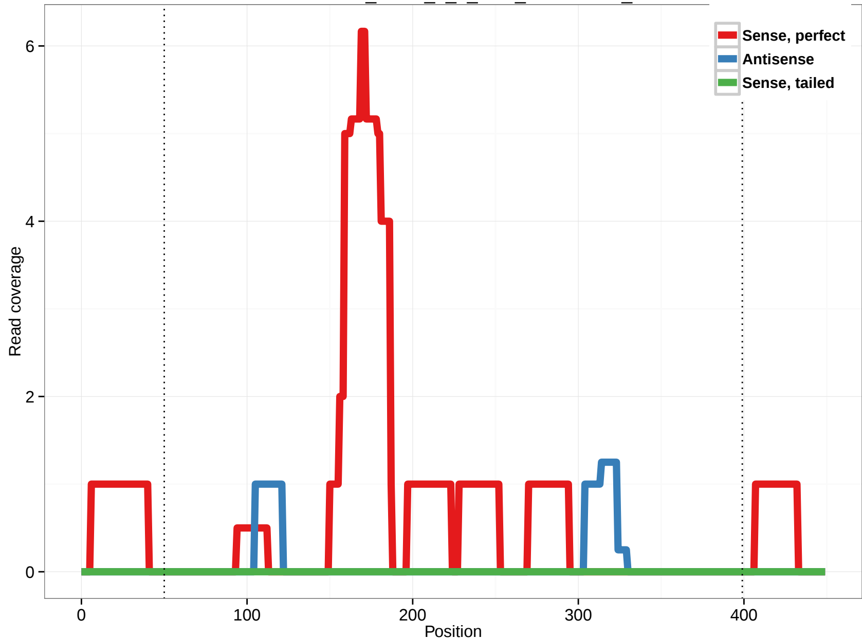
uc009wer.2_intron_0_0_chr1_109191614_r
