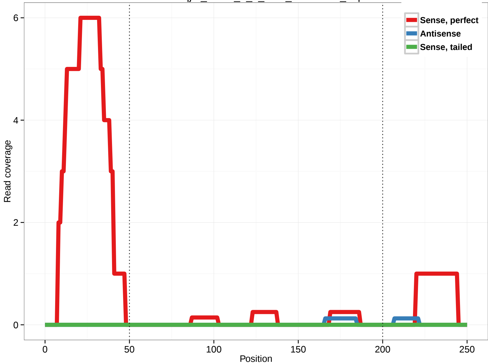
uc009vqj.1_intron_5_0_chr1_23208977_f.5p
