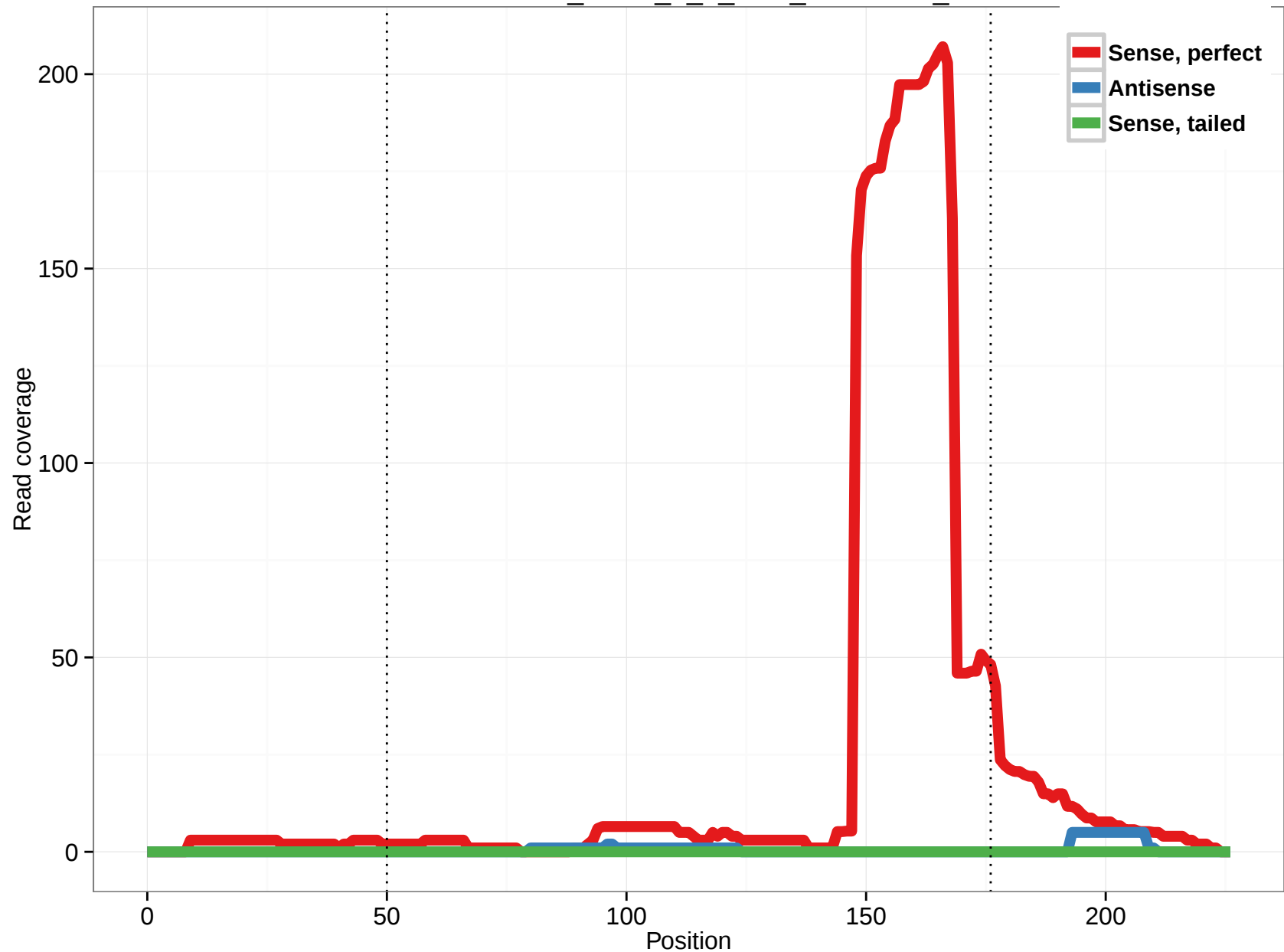
uc009vod.1_intron_2_0_chr1_14104993_f
