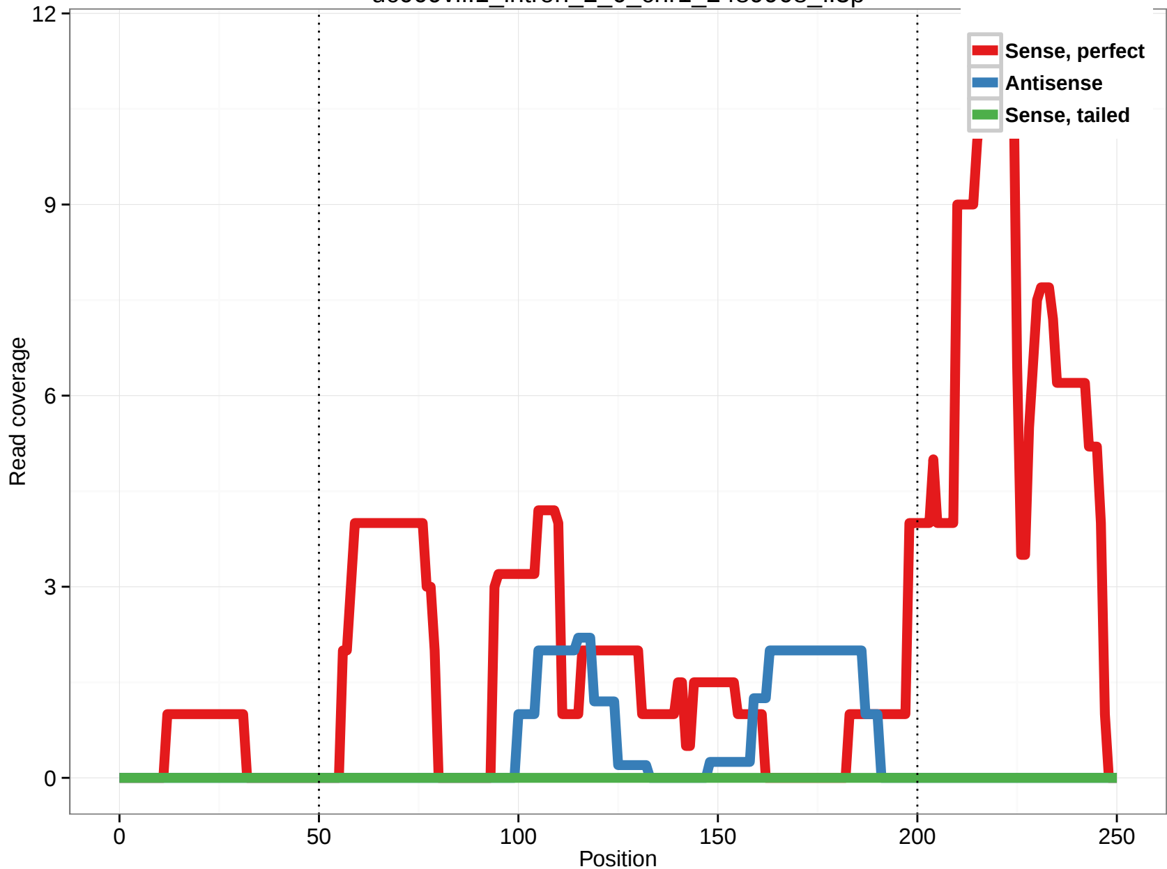
uc009vlf.1_intron_2_0_chr1_2489908_f.3p
