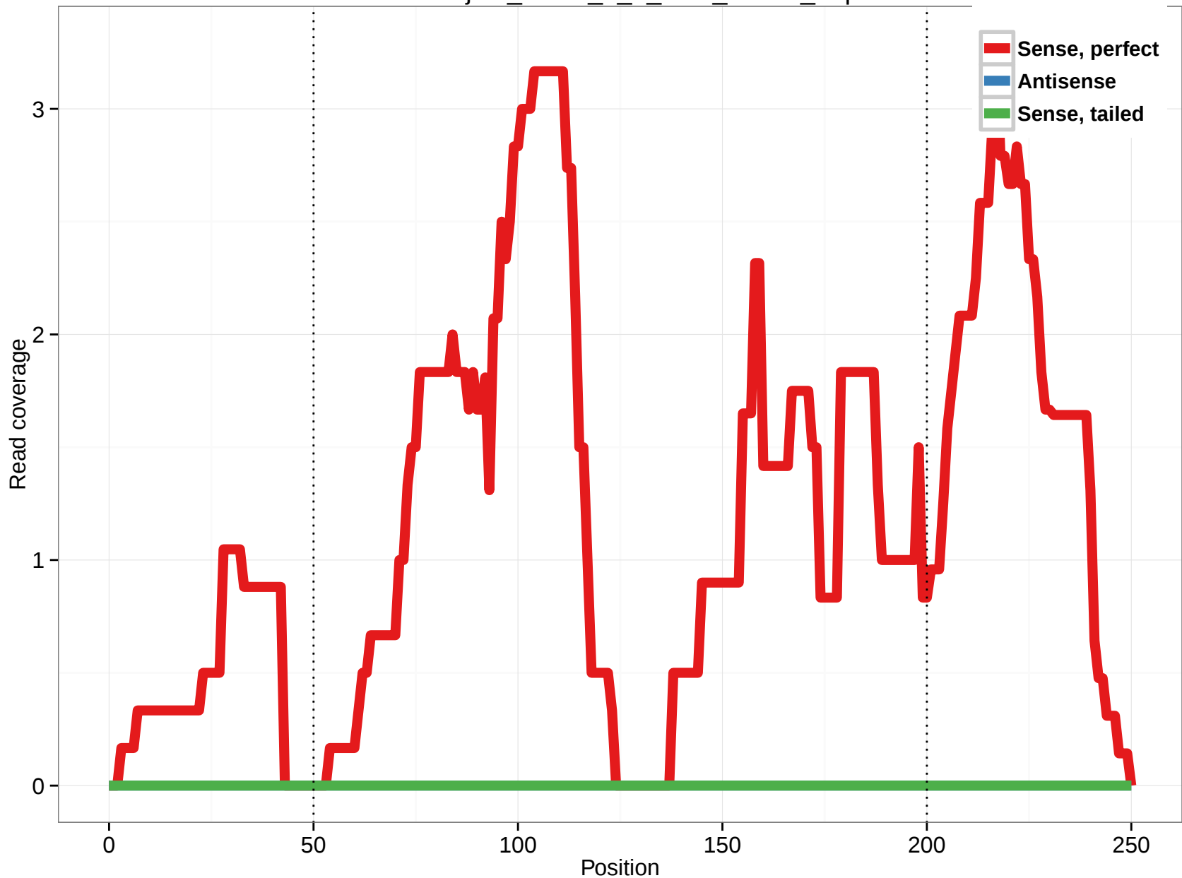
uc009vjb.1_intron_5_0_chr1_24892_r.3p
