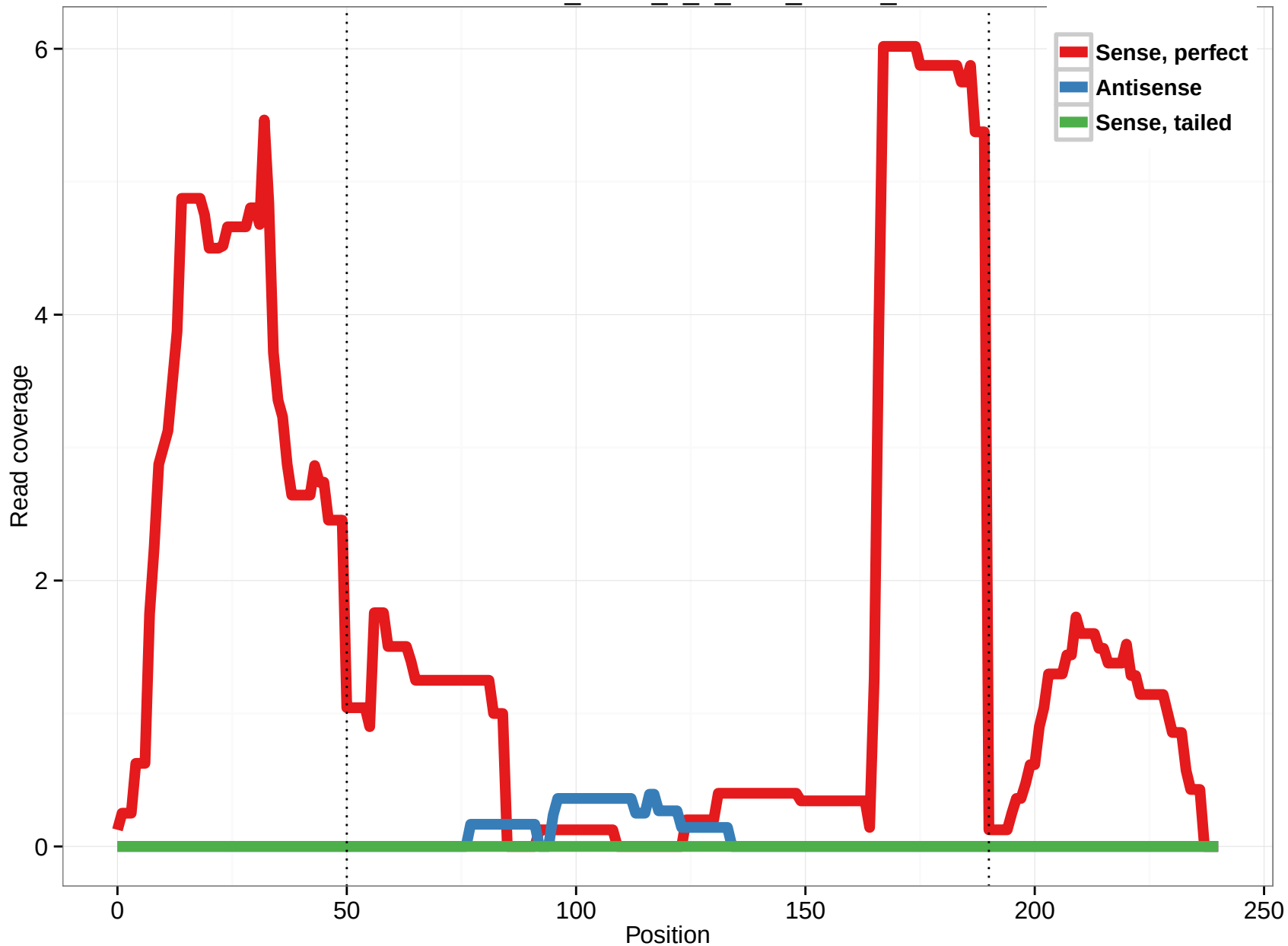
uc009vis.2_intron_0_0_chr1_14830_r
