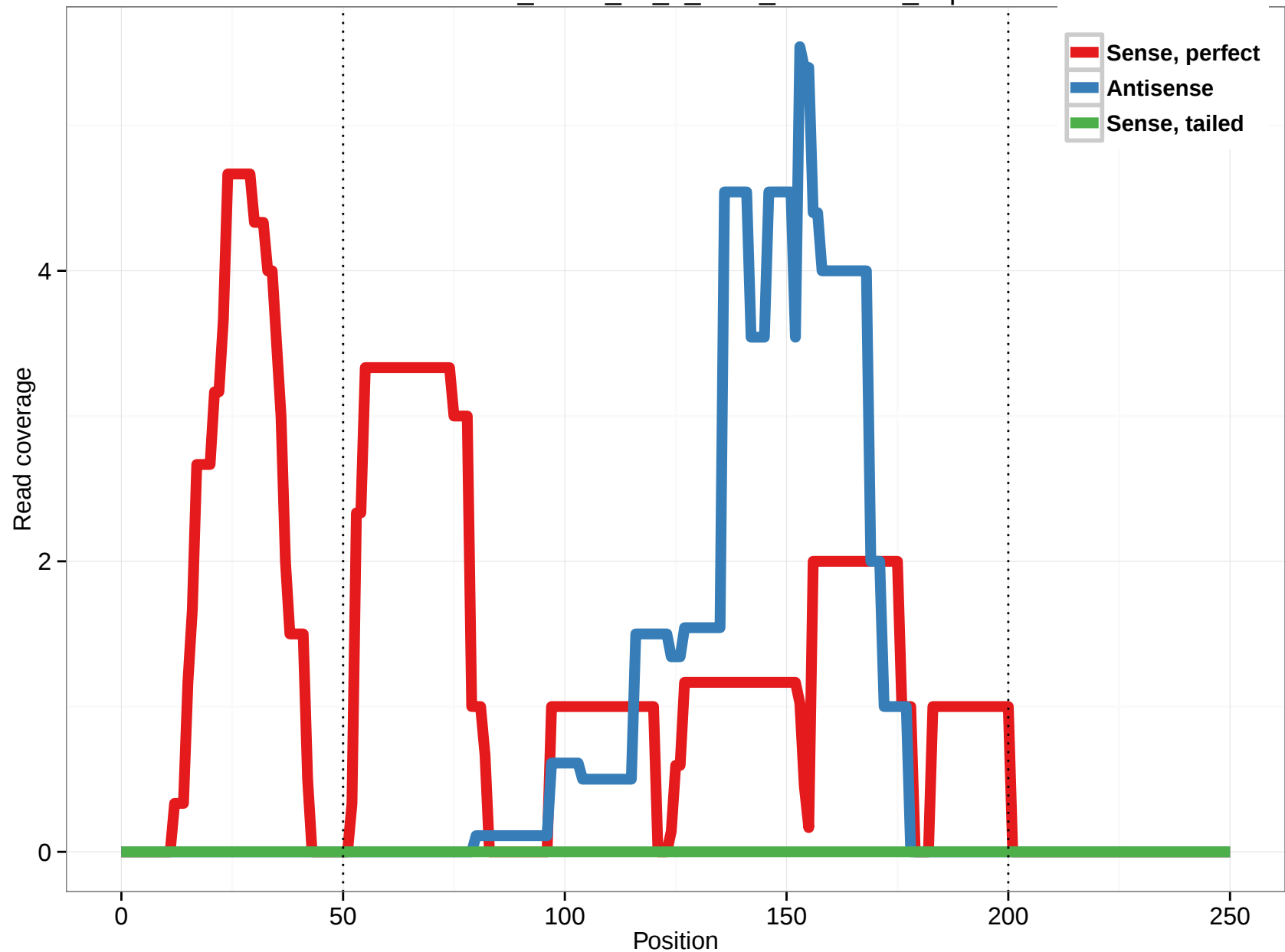
uc004fst.1_intron_29_0_chrY_14923717_f.5p
