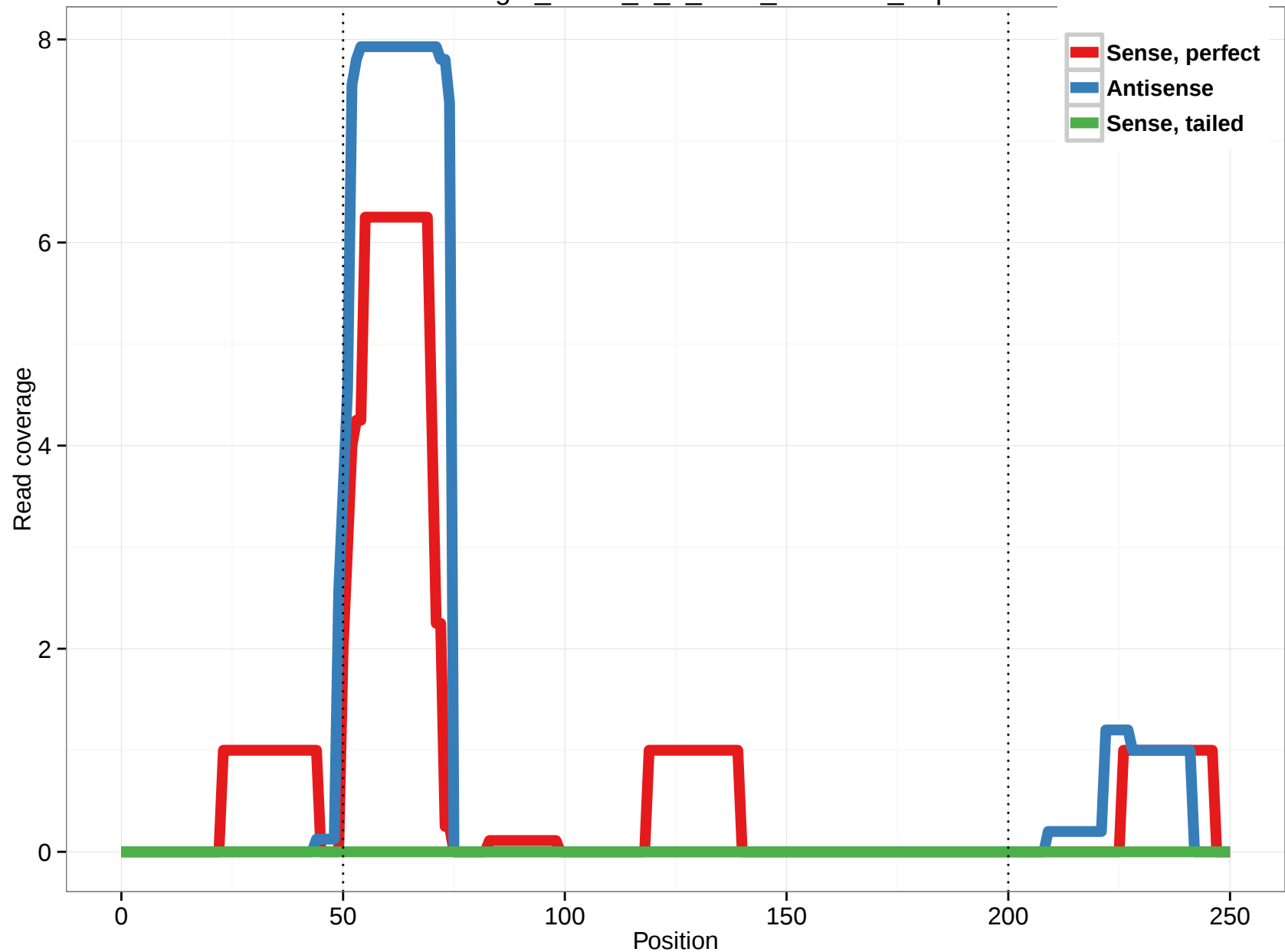
uc004frg.2_intron_2_0_chrY_7645070_r.3p
