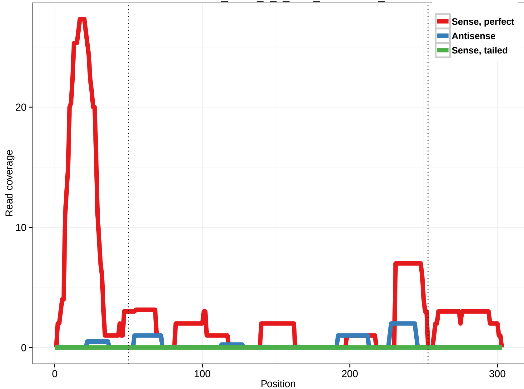
uc004flo.2_intron_2_0_chrX_153714673_r
