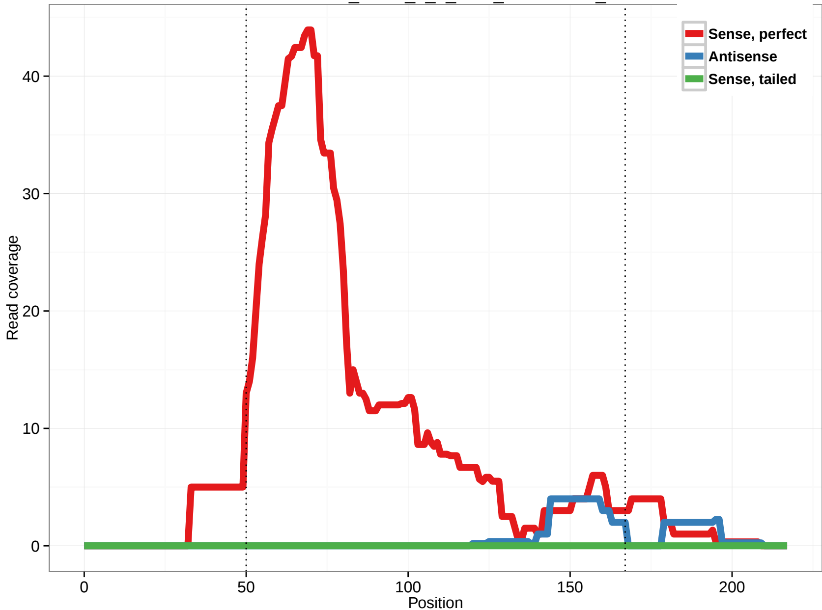
uc004fkx.2_intron_7_0_chrX_153648434_f
