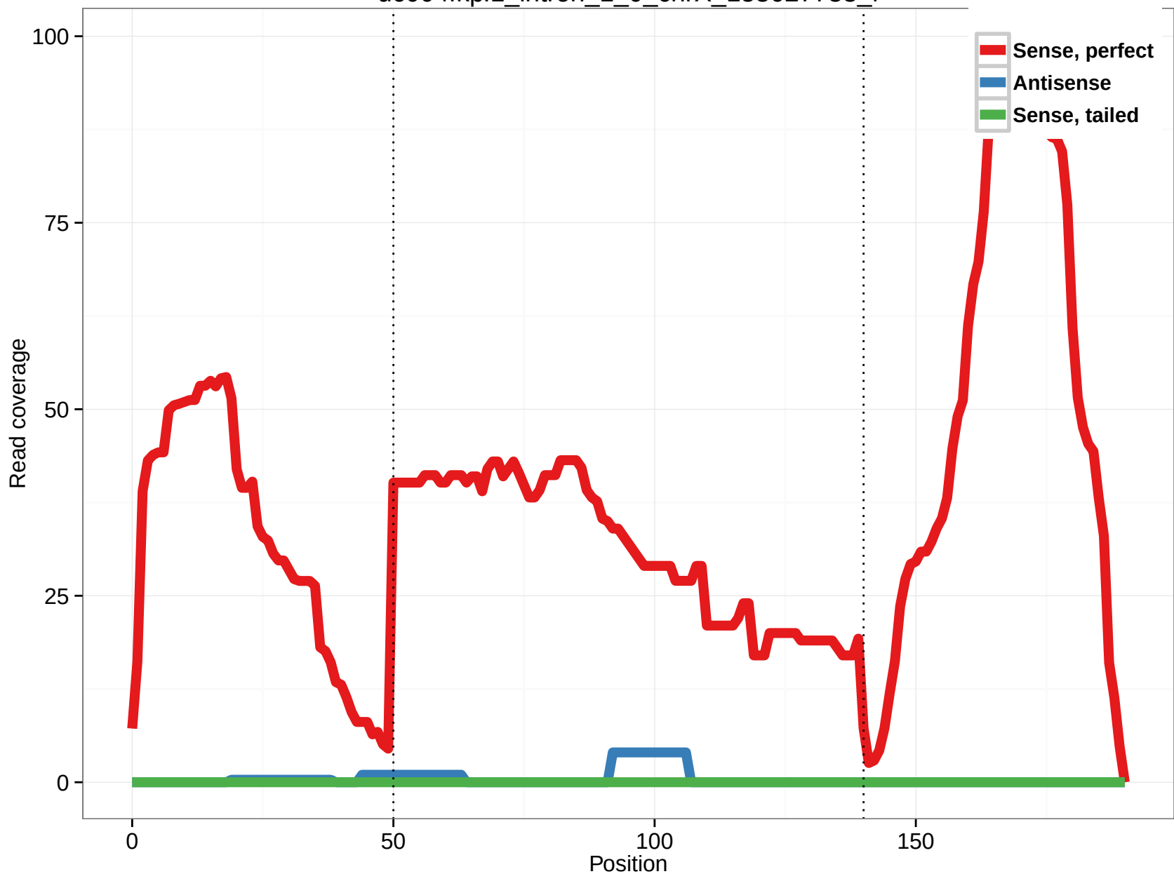
uc004fkp.1_intron_1_0_chrX_153627738_f
