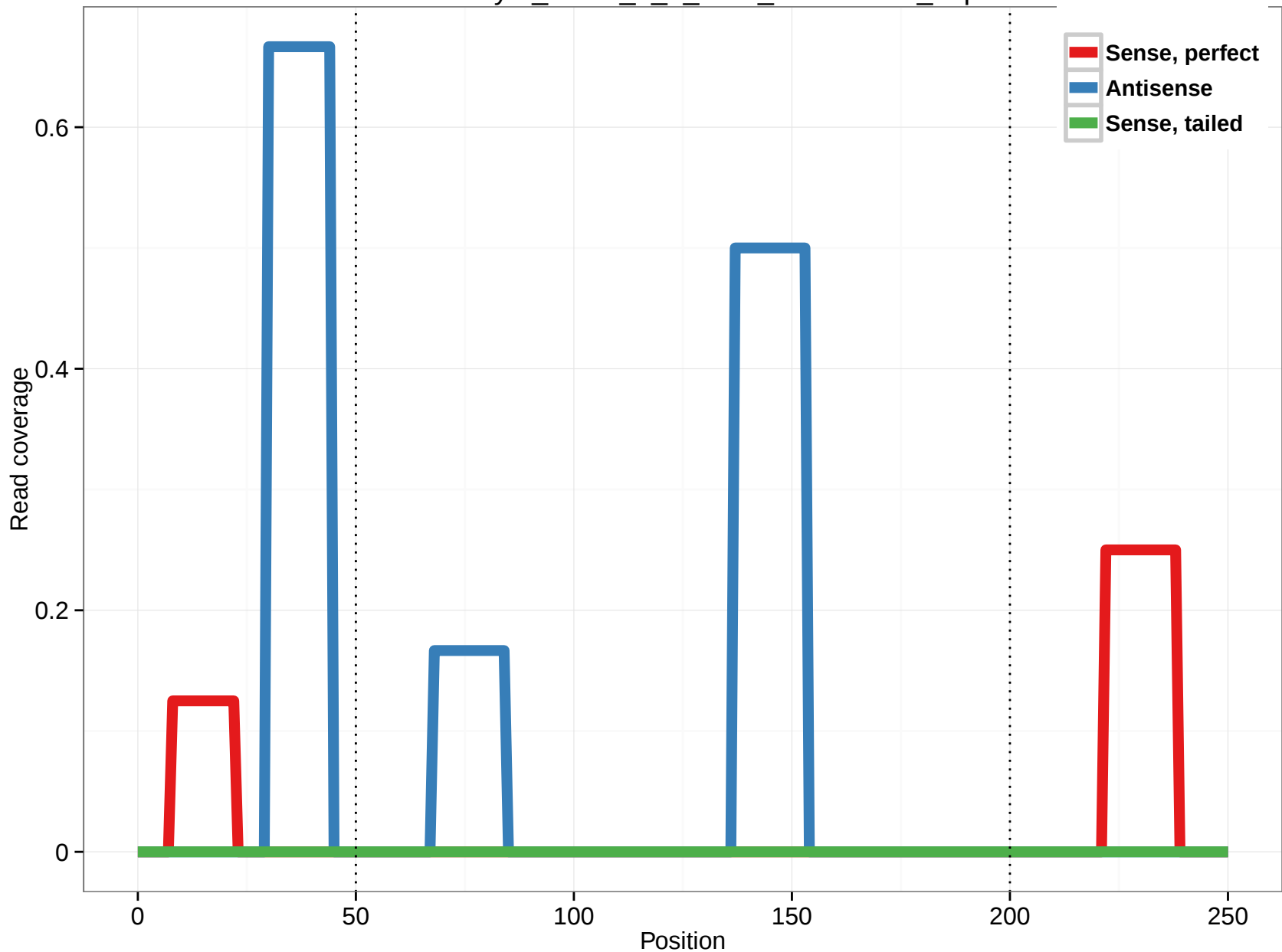
uc004ezy.2_intron_0_0_chrX_135614456_f.3p
