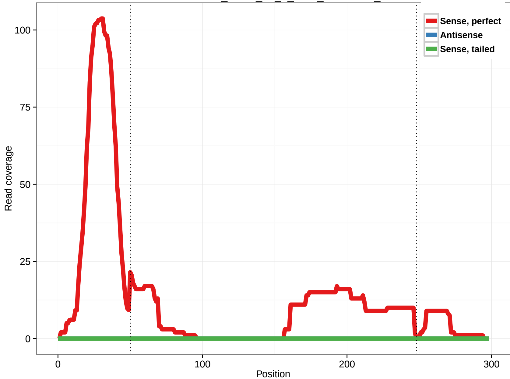
uc004dzo.2_intron_10_0_chrX_70518359_f
