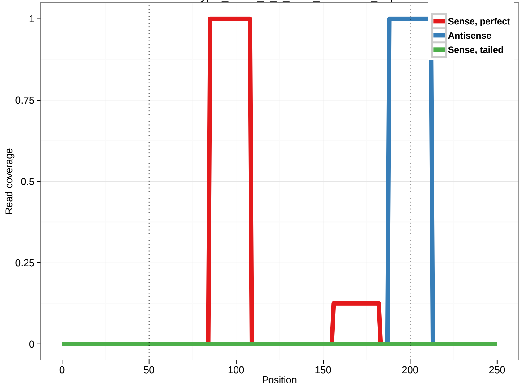
uc004dyp.1_intron_1_0_chrX_70256218_r.3p
