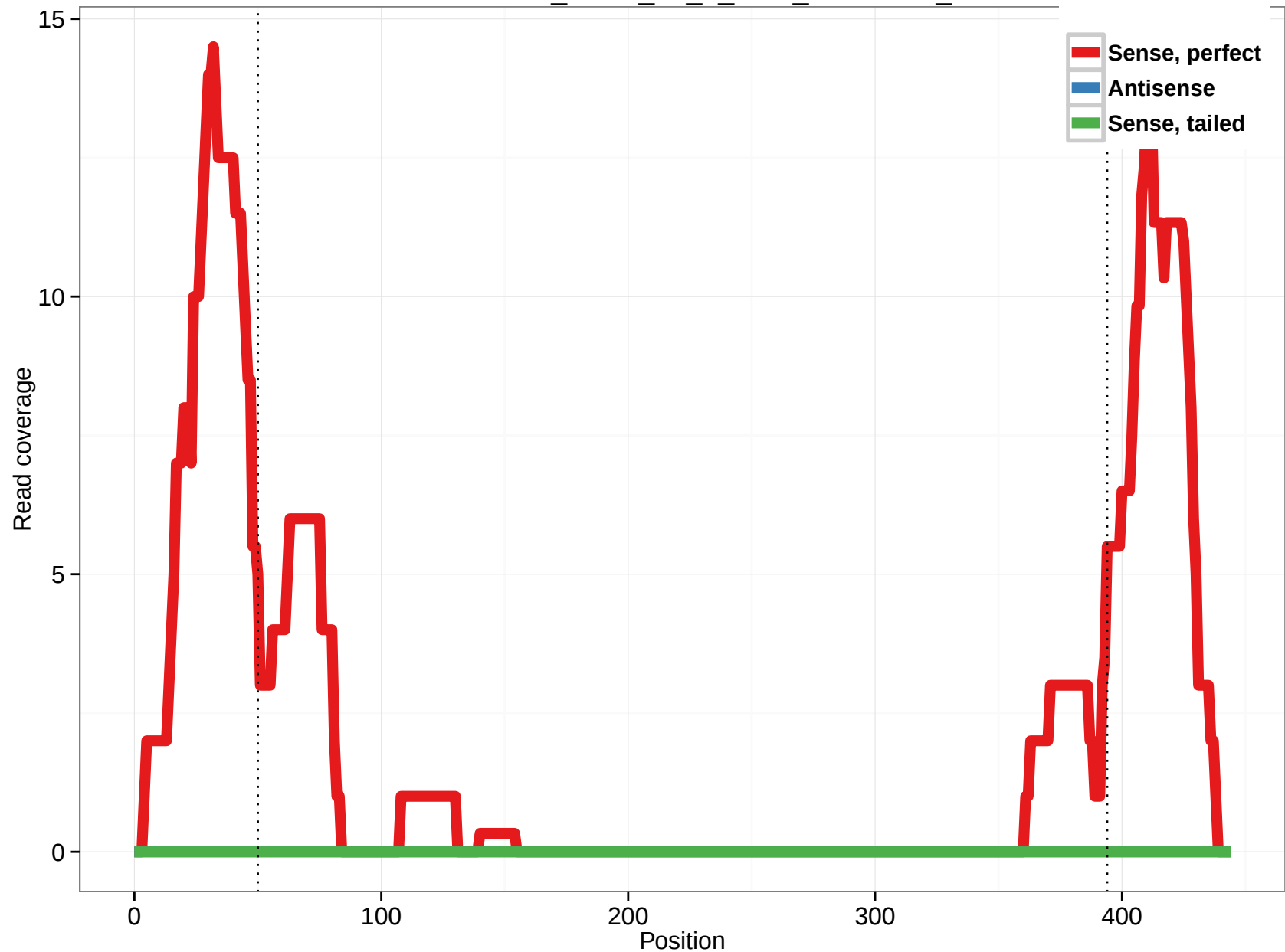
uc004dsn.2_intron_33_0_chrX_53591684_r
