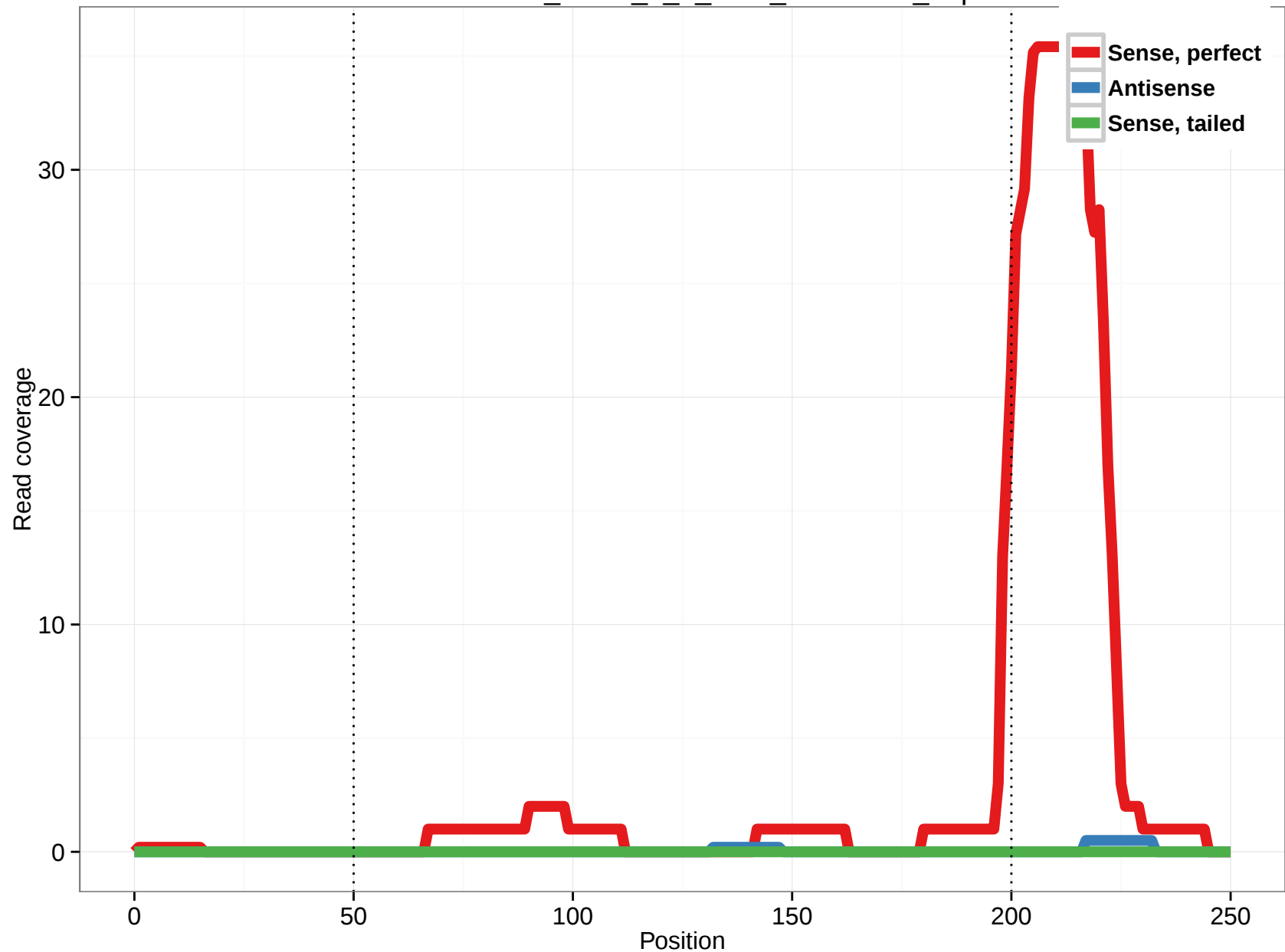
uc004dmb.3_intron_0_0_chrX_48888113_r.3p
