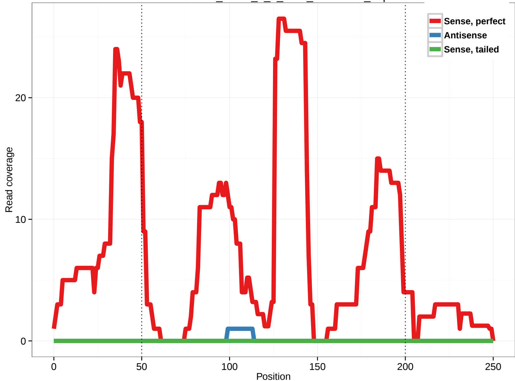
uc004dks.1_intron_0_0_chrX_48660550_f.5p
