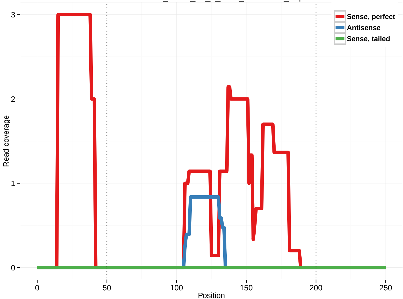
uc004dfk.3_intron_14_0_chrX_41448846_r.5p
