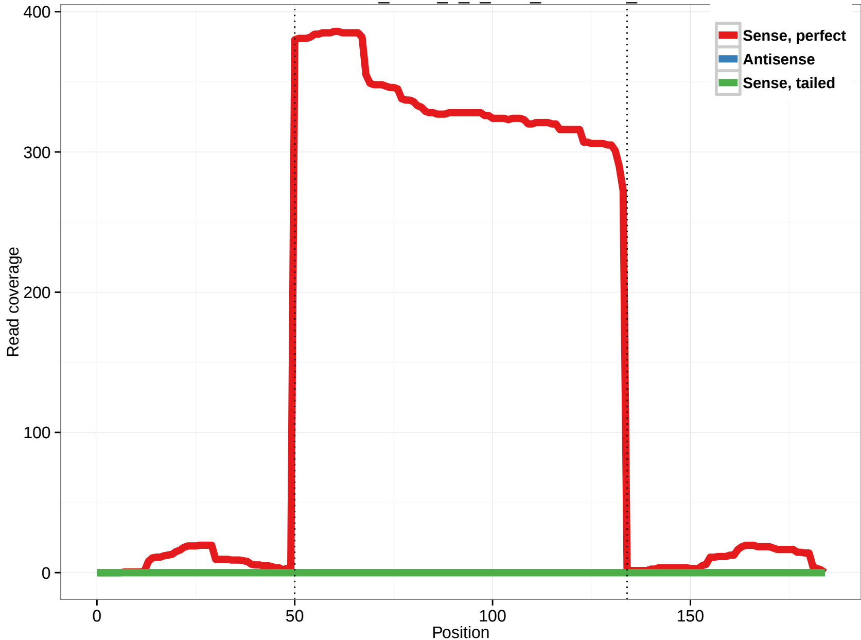
uc004dbc.2_intron_2_0_chrX_24075666_f
