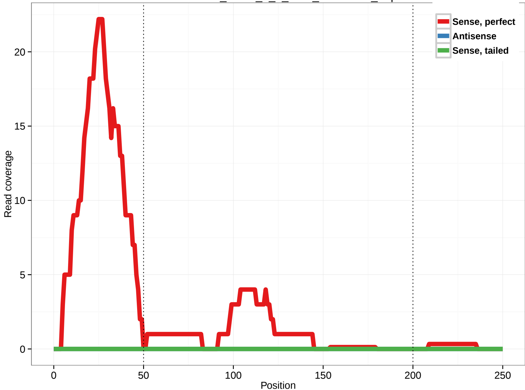
uc004dao.2_intron_5_0_chrX_23724857_r.5p
