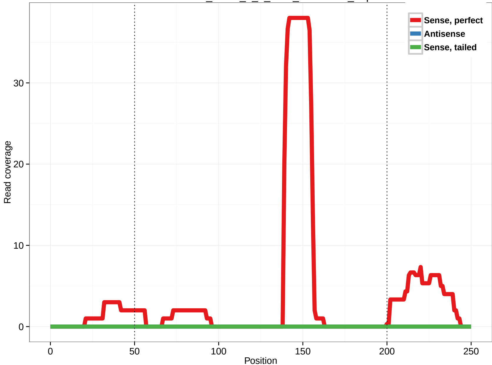
uc004dao.2_intron_5_0_chrX_23724857_r.3p
