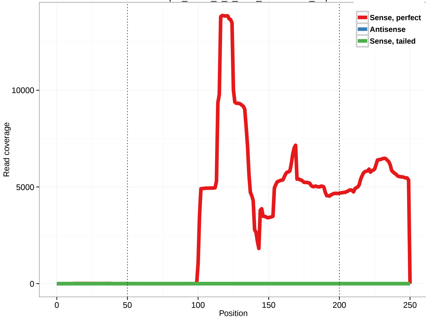
uc004cip.3_intron_1_0_chr9_139619563_r.5p
