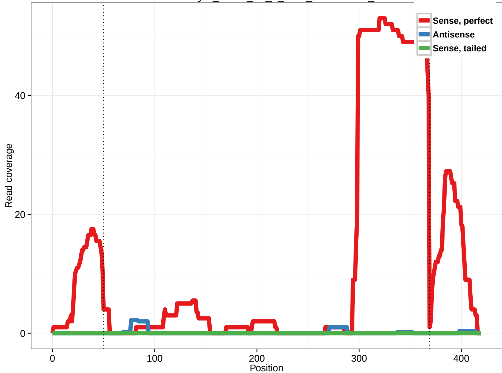
uc004cey.2_intron_10_0_chr9_137020496_f
