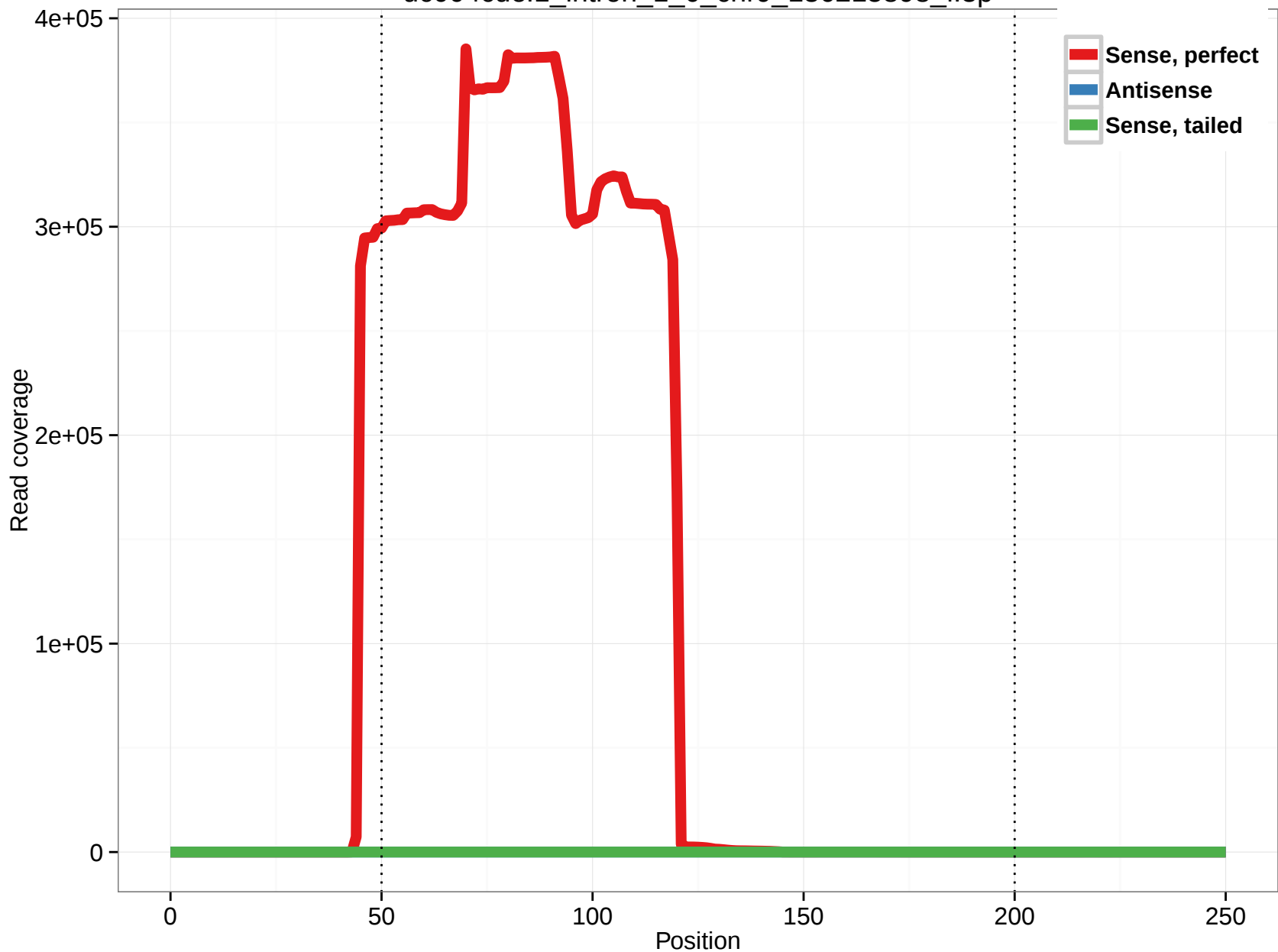
uc004cde.1_intron_1_0_chr9_136215898_f.3p
