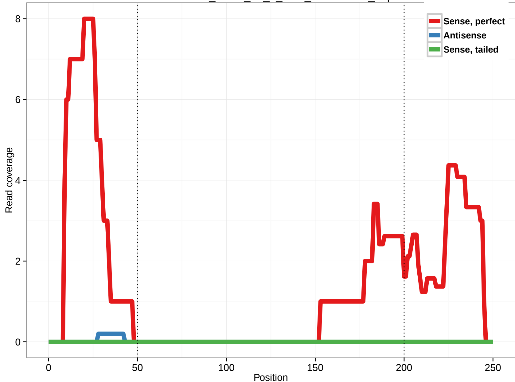
uc004bws.1_intron_11_0_chr9_131735529_f.5p
