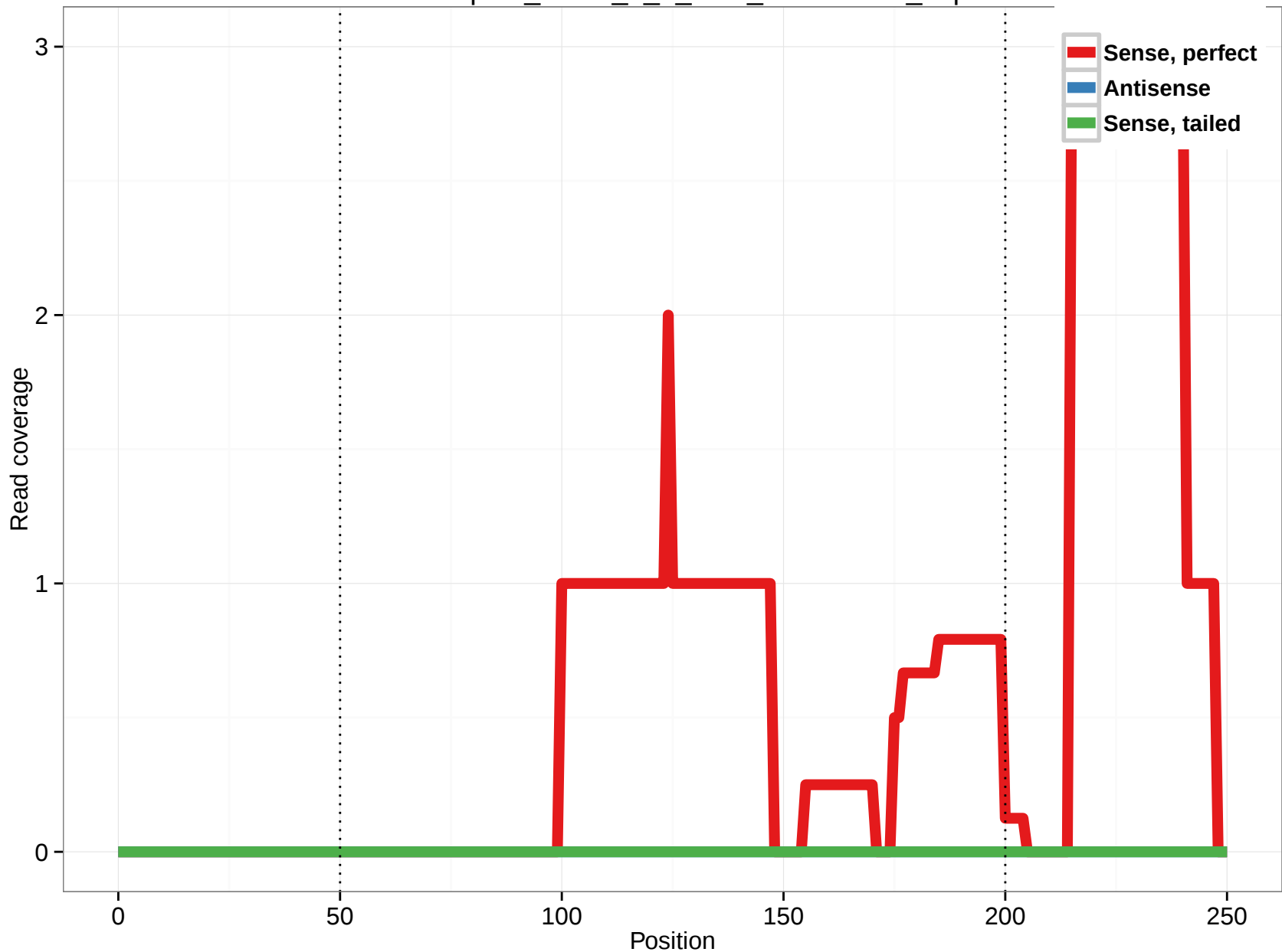
uc004bpo.2_intron_3_0_chr9_128061386_f.3p
