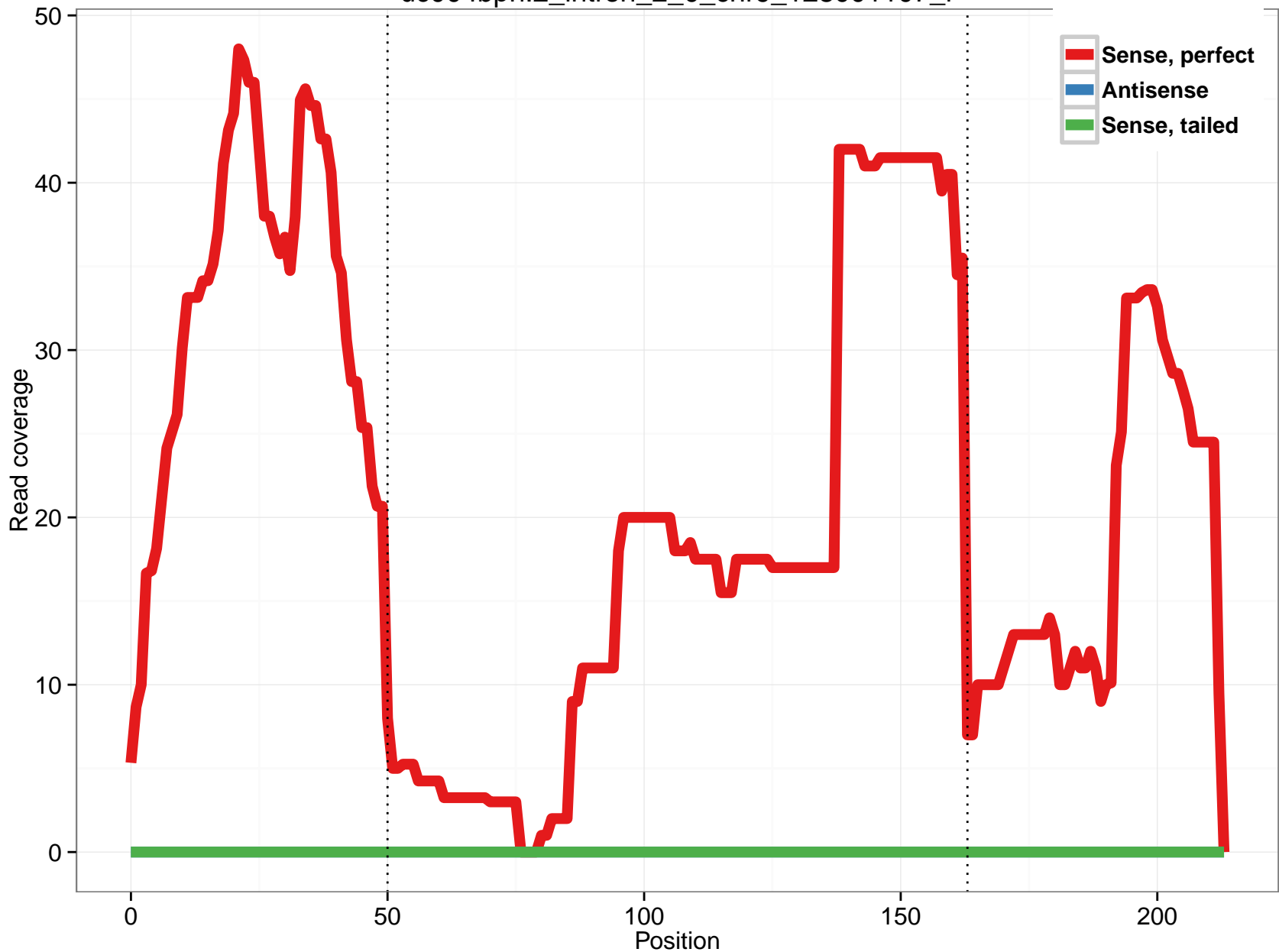
uc004bpn.2_intron_2_0_chr9_128001107_r
