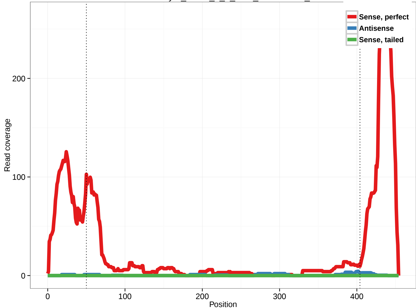
uc004boy.1_intron_2_0_chr9_127623835_r
