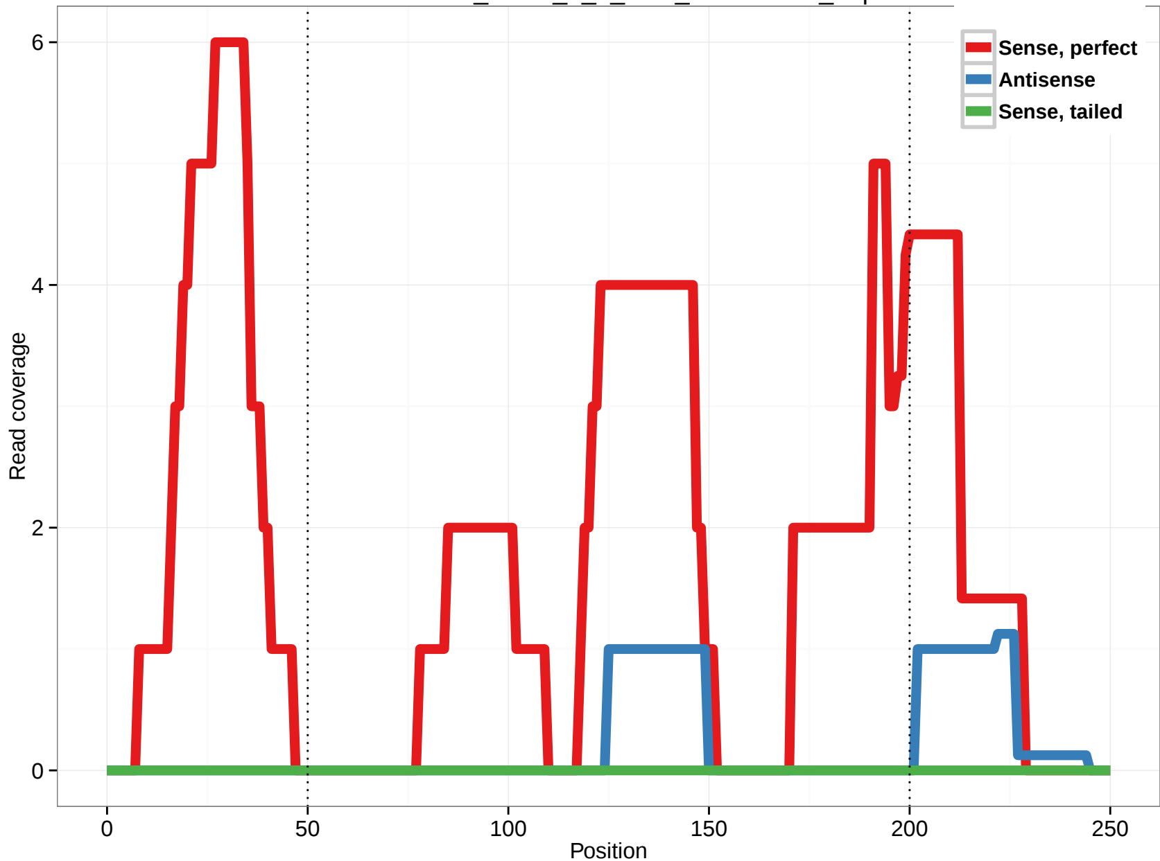
uc004bns.2_intron_6_0_chr9_125909334_r.5p
