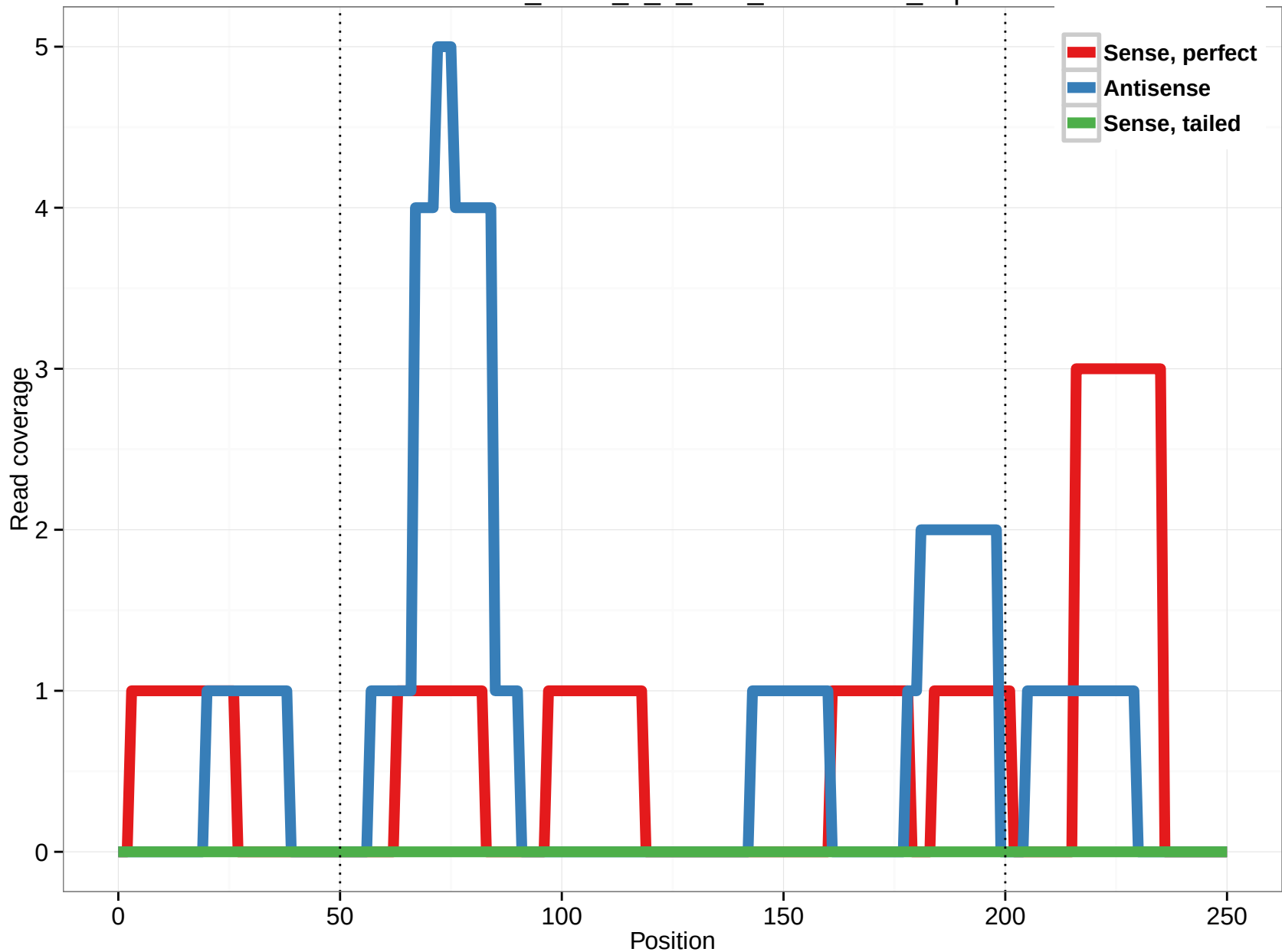
uc004bdn.2_intron_0_0_chr9_111696846_f.5p
