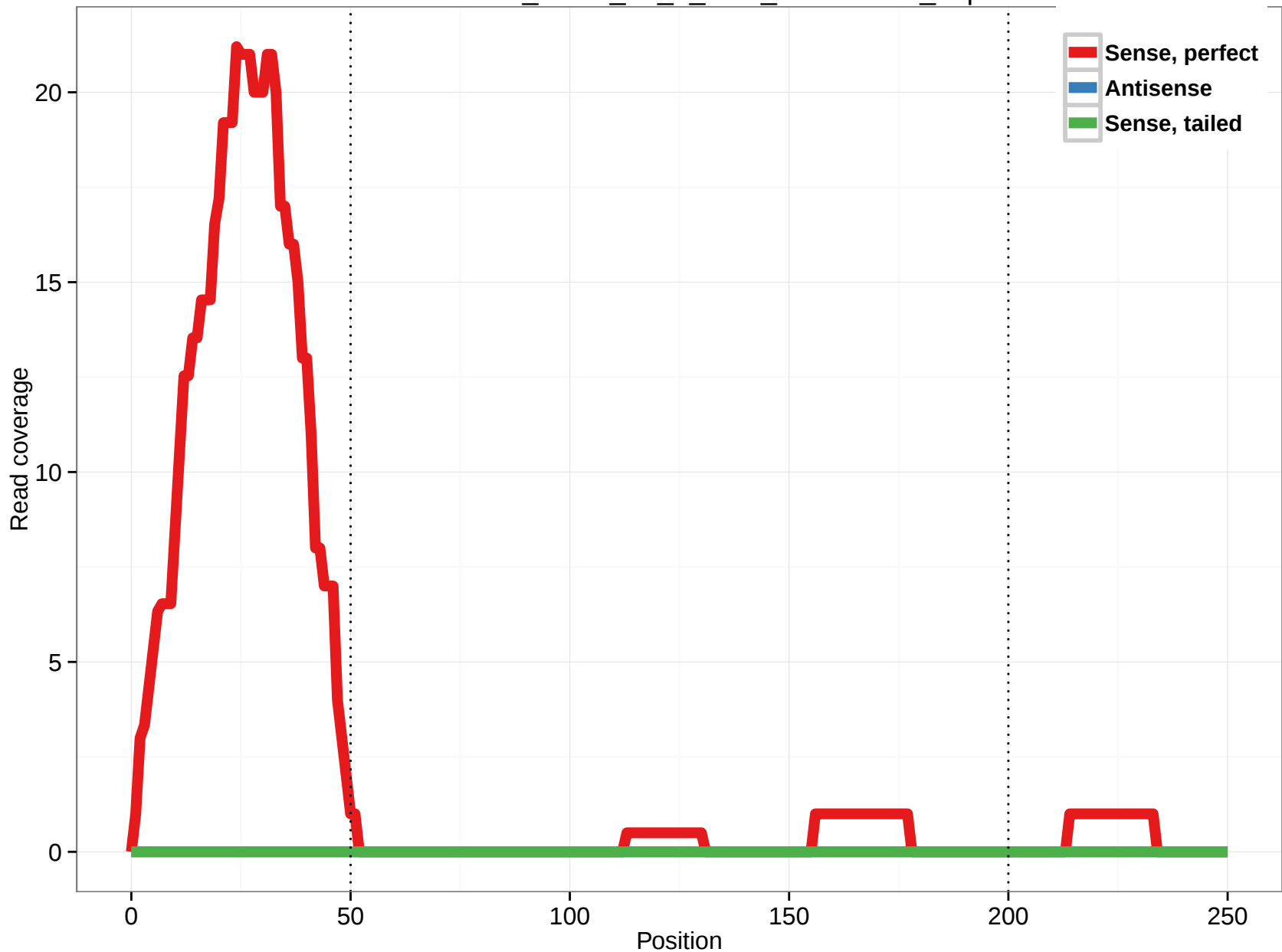
uc004bcz.2_intron_10_0_chr9_109765708_f.5p
