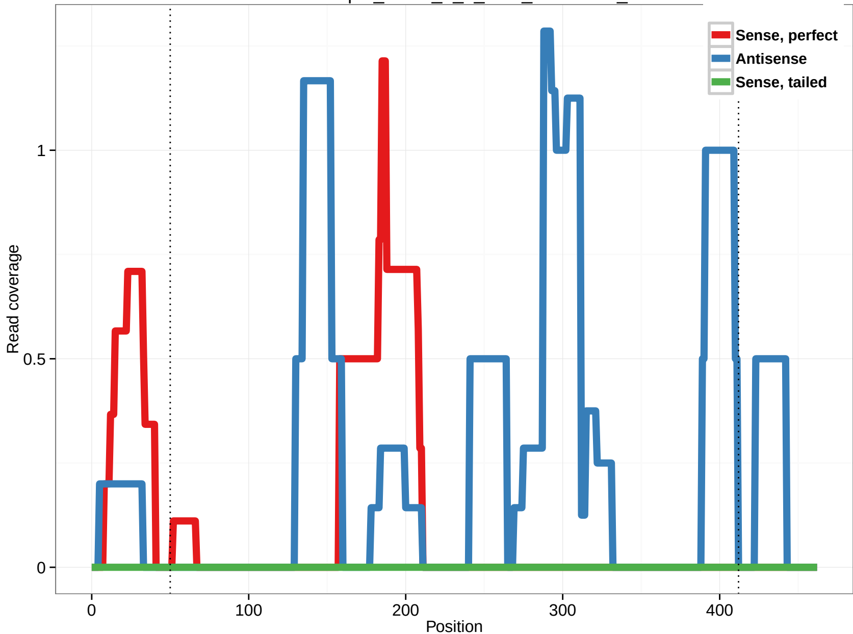
uc004aup.1_intron_0_0_chr9_97081533_r
