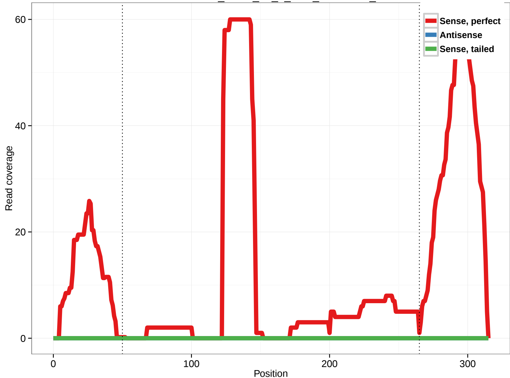
uc004ars.1_intron_30_0_chr9_95050193_r
