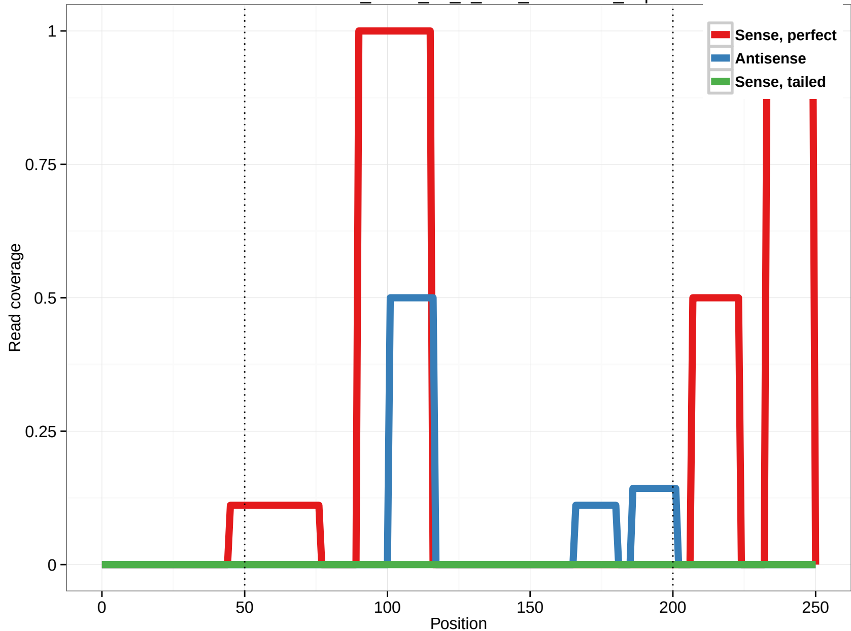
uc004anz.1_intron_13_0_chr9_87367001_f.3p
