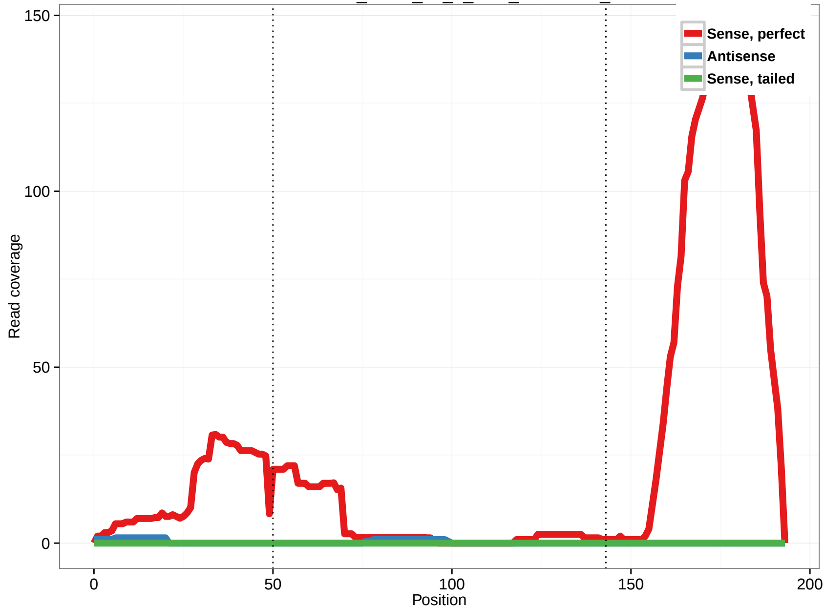
uc004ank.3_intron_13_0_chr9_86593195_r
