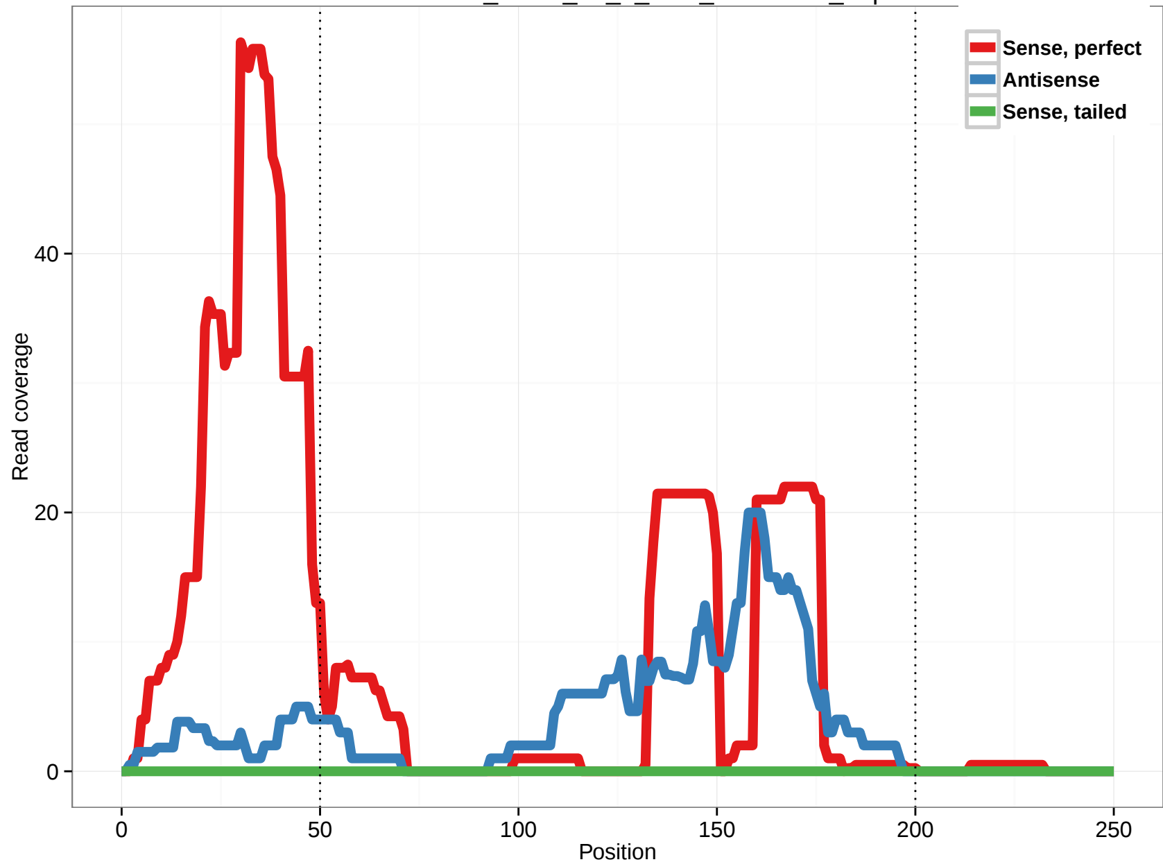
uc004ana.2_intron_16_0_chr9_86530594_r.5p
